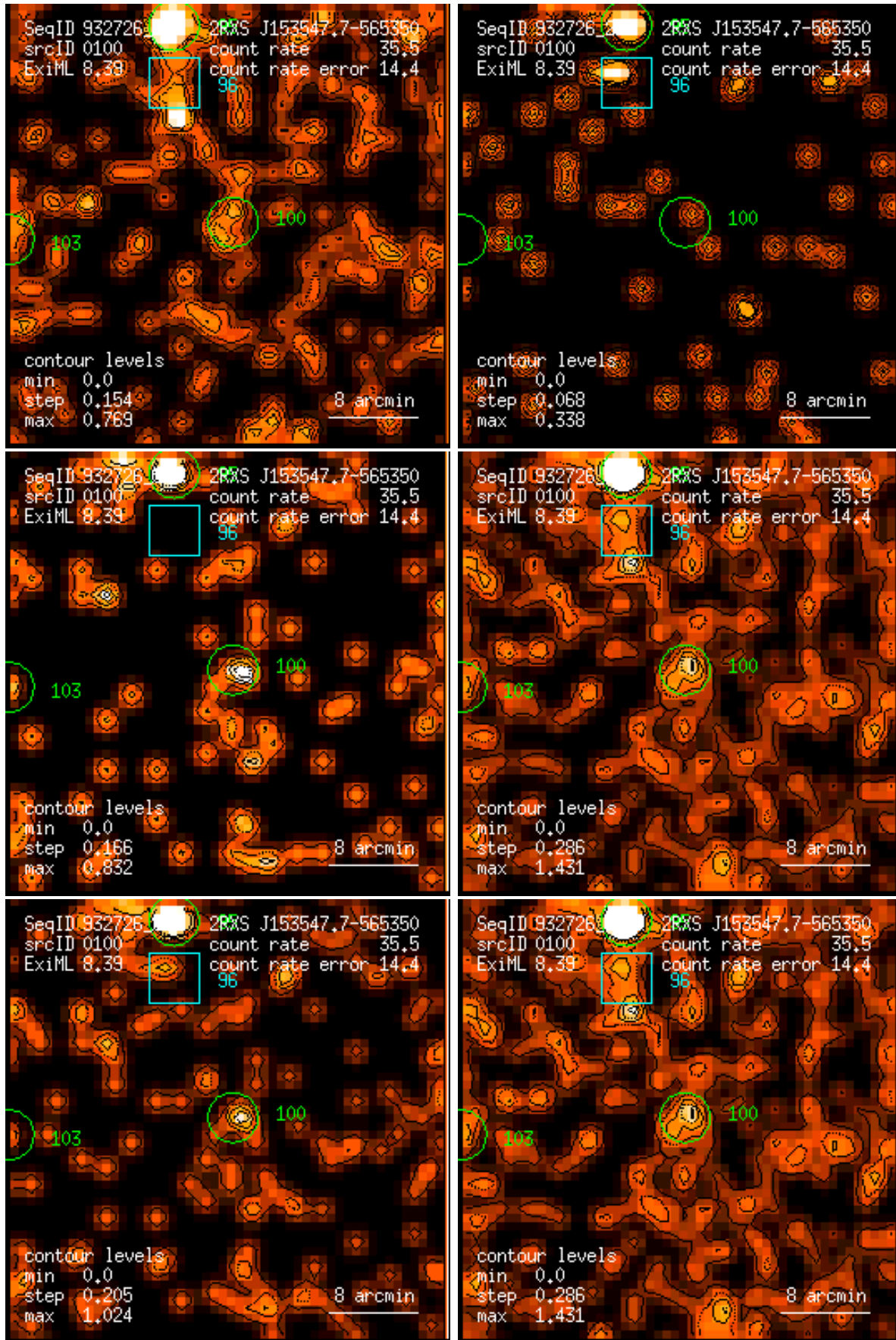
Figure 100: RASS 932726: detection 0100: band rate images, Gaussian filter: (1) PSPC channels 11 – 41, (2) 52 – 90, (3) 91 – 201, (4) 11 – 235, (5) 52 – 201, (6) 11 – 201. Broad band rates in counts/ks. Band rate contour levels in counts/ks/arcmin 2 .
