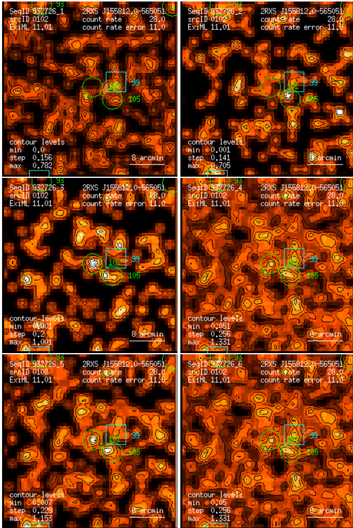
Figure 102: RASS 932726: detection 0102: band rate images, Gaussian filter: (1) PSPC channels 11 – 41, (2) 52 – 90, (3) 91 – 201, (4) 11 – 235, (5) 52 – 201, (6) 11 – 201. Broad band rates in counts/ks. Band rate contour levels in counts/ks/arcmin 2 .
