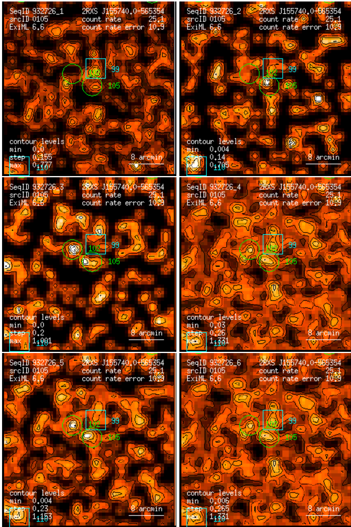
Figure 105: RASS 932726: detection 0105: band rate images, Gaussian filter: (1) PSPC channels 11 – 41, (2) 52 – 90, (3) 91 – 201, (4) 11 – 235, (5) 52 – 201, (6) 11 – 201. Broad band rates in counts/ks. Band rate contour levels in counts/ks/arcmin 2 .
