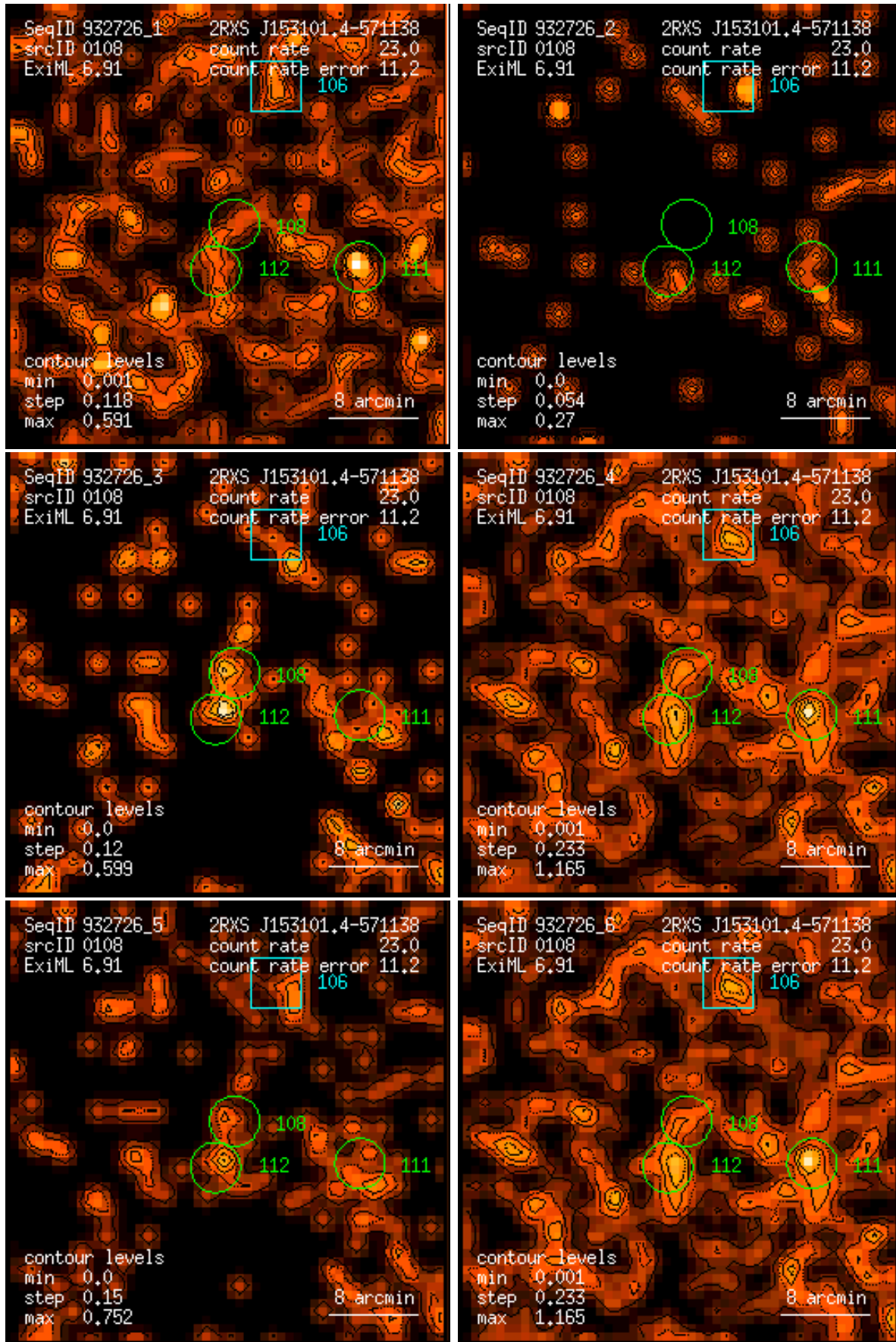
Figure 108: RASS 932726: detection 0108: band rate images, Gaussian filter: (1) PSPC channels 11 – 41, (2) 52 – 90, (3) 91 – 201, (4) 11 – 235, (5) 52 – 201, (6) 11 – 201. Broad band rates in counts/ks. Band rate contour levels in counts/ks/arcmin 2 .
