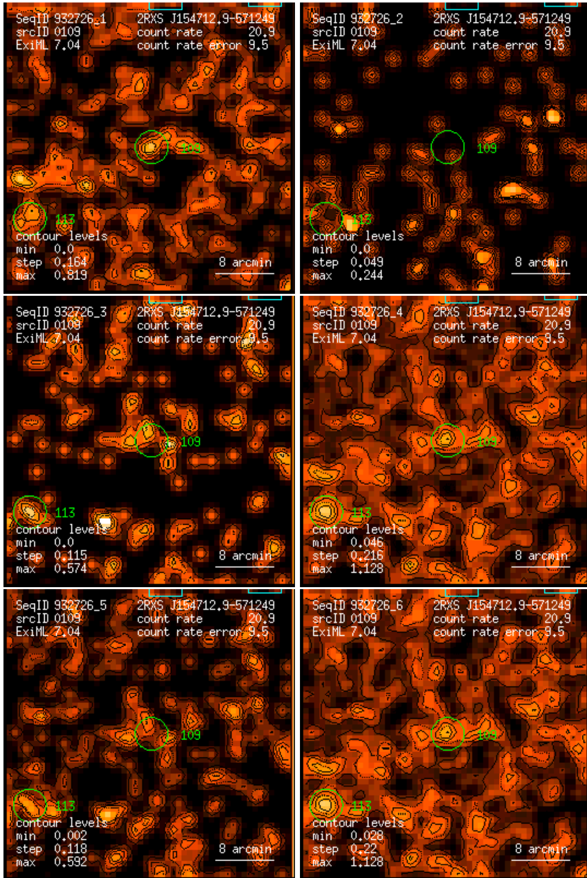
Figure 109: RASS 932726: detection 0109: band rate images, Gaussian filter: (1) PSPC channels 11 – 41, (2) 52 – 90, (3) 91 – 201, (4) 11 – 235, (5) 52 – 201, (6) 11 – 201. Broad band rates in counts/ks. Band rate contour levels in counts/ks/arcmin 2 .
