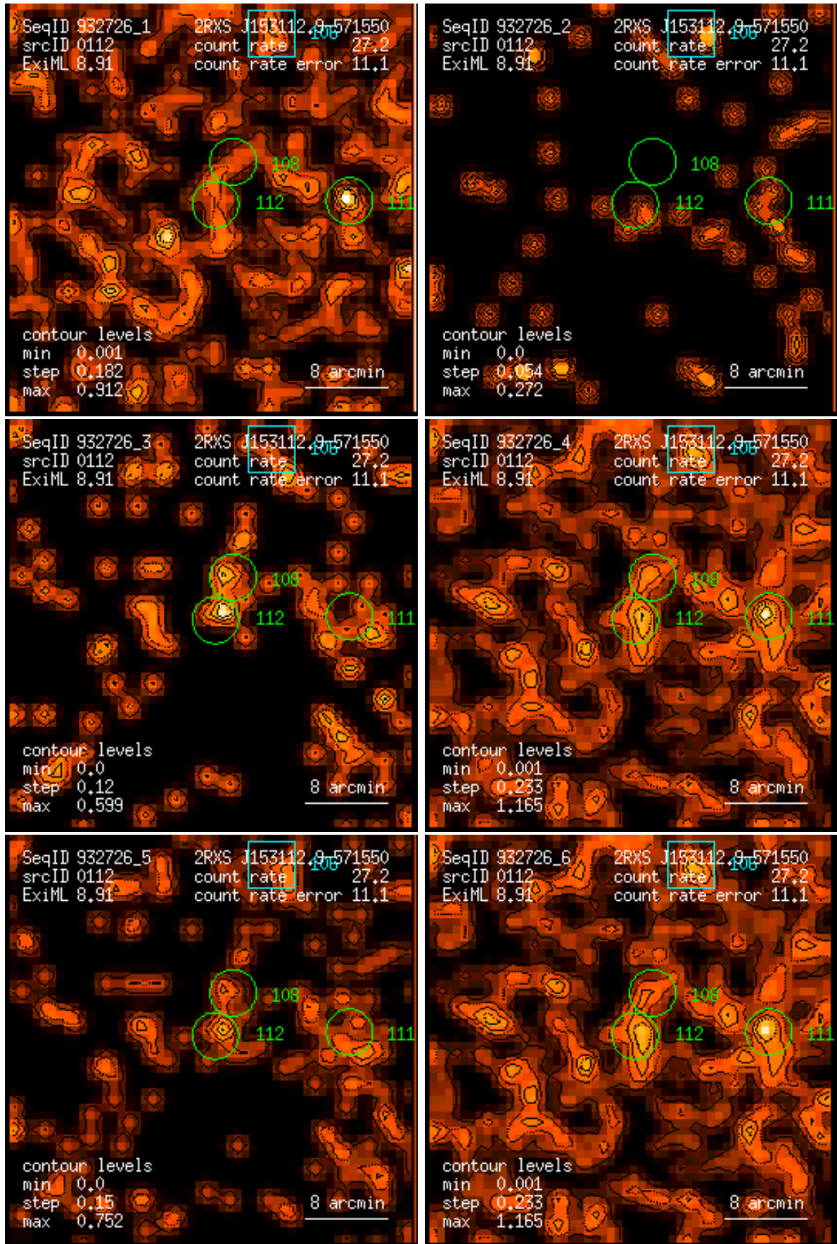
Figure 112: RASS 932726: detection 0112: band rate images, Gaussian filter: (1) PSPC channels 11 – 41, (2) 52 – 90, (3) 91 – 201, (4) 11 – 235, (5) 52 – 201, (6) 11 – 201. Broad band rates in counts/ks. Band rate contour levels in counts/ks/arcmin 2 .
