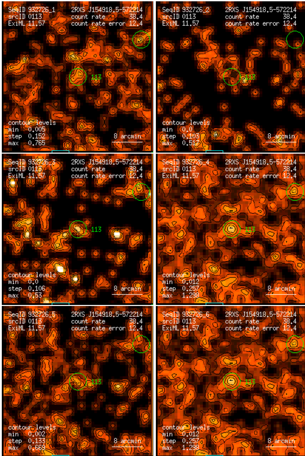
Figure 113: RASS 932726: detection 0113: band rate images, Gaussian filter: (1) PSPC channels 11 – 41, (2) 52 – 90, (3) 91 – 201, (4) 11 – 235, (5) 52 – 201, (6) 11 – 201. Broad band rates in counts/ks. Band rate contour levels in counts/ks/arcmin 2 .
