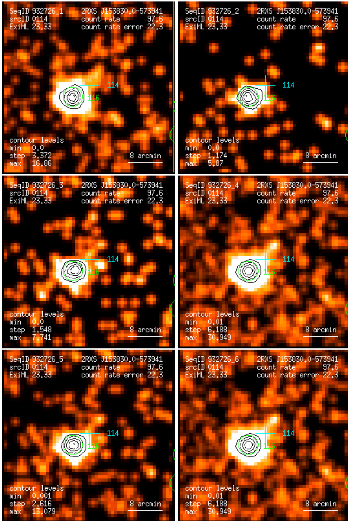
Figure 114: RASS 932726: detection 0114: band rate images, Gaussian filter: (1) PSPC channels 11 – 41, (2) 52 – 90, (3) 91 – 201, (4) 11 – 235, (5) 52 – 201, (6) 11 – 201. Broad band rates in counts/ks. Band rate contour levels in counts/ks/arcmin 2 .
