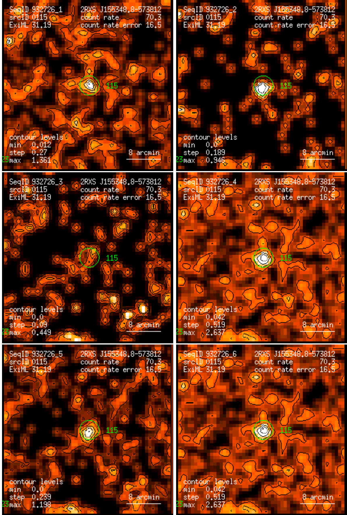
Figure 115: RASS 932726: detection 0115: band rate images, Gaussian filter: (1) PSPC channels 11 – 41, (2) 52 – 90, (3) 91 – 201, (4) 11 – 235, (5) 52 – 201, (6) 11 – 201. Broad band rates in counts/ks. Band rate contour levels in counts/ks/arcmin 2 .
