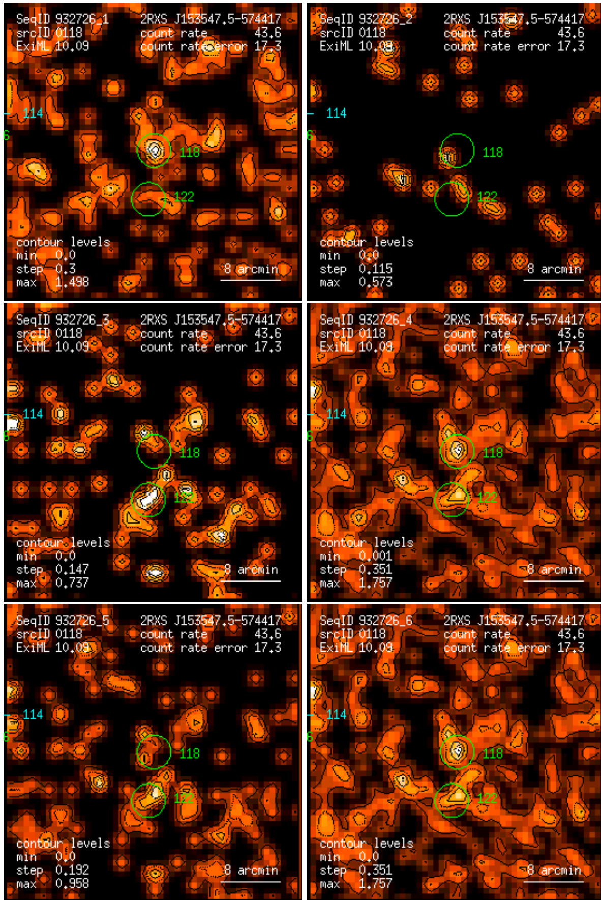
Figure 118: RASS 932726: detection 0118: band rate images, Gaussian filter: (1) PSPC channels 11 – 41, (2) 52 – 90, (3) 91 – 201, (4) 11 – 235, (5) 52 – 201, (6) 11 – 201. Broad band rates in counts/ks. Band rate contour levels in counts/ks/arcmin 2 .
