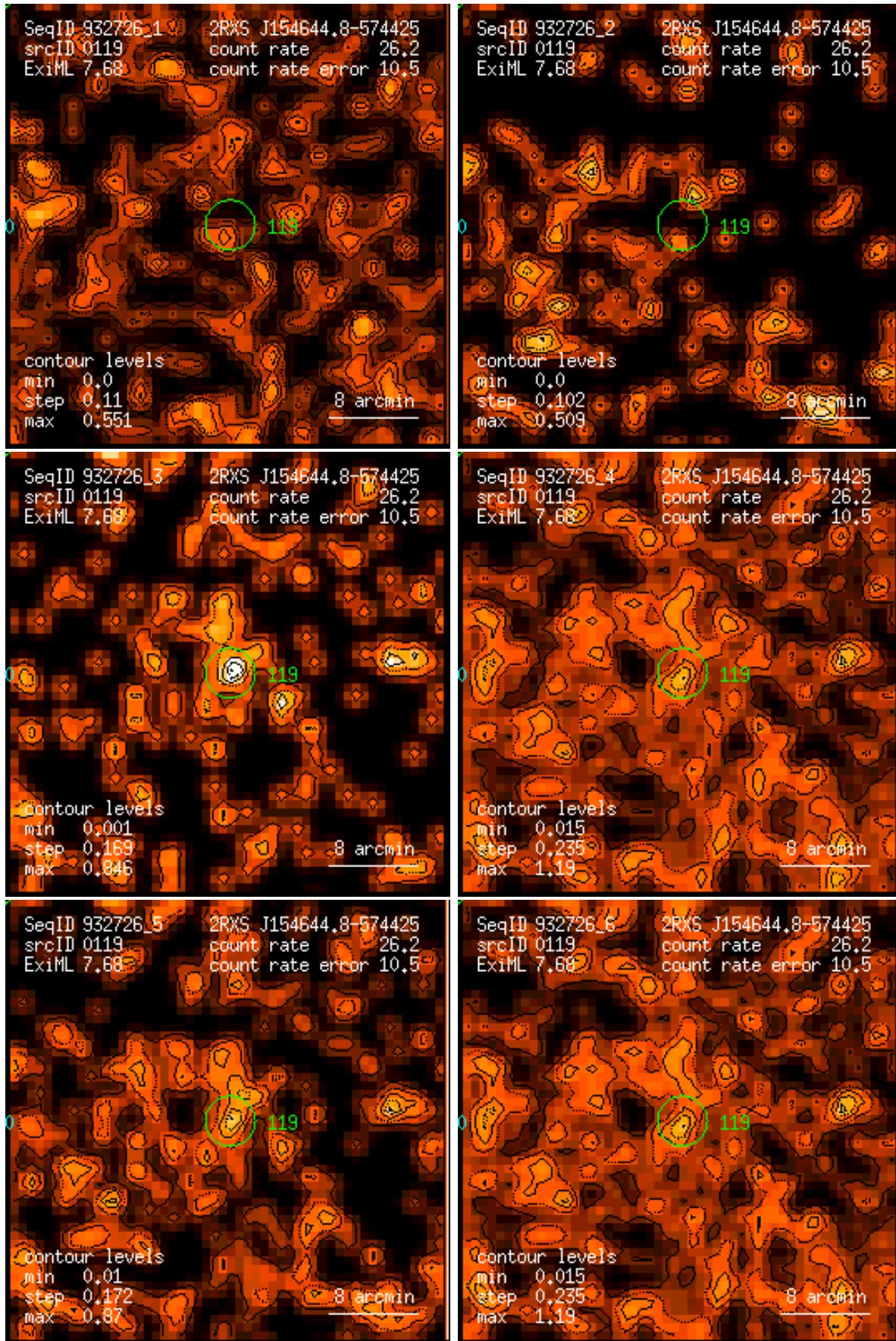
Figure 119: RASS 932726: detection 0119: band rate images, Gaussian filter: (1) PSPC channels 11 – 41, (2) 52 – 90, (3) 91 – 201, (4) 11 – 235, (5) 52 – 201, (6) 11 – 201. Broad band rates in counts/ks. Band rate contour levels in counts/ks/arcmin 2 .
