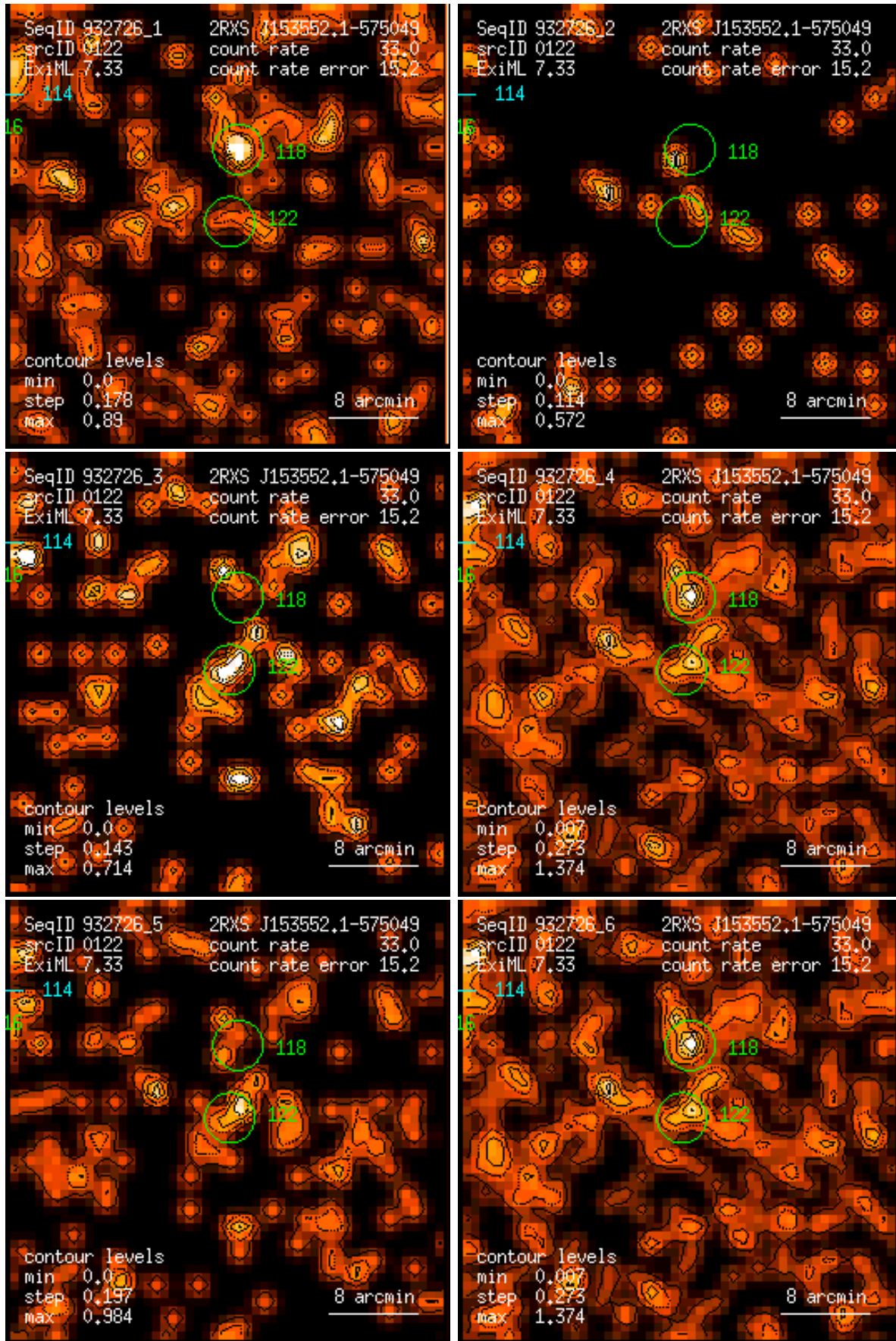
Figure 122: RASS 932726: detection 0122: band rate images, Gaussian filter: (1) PSPC channels 11 – 41, (2) 52 – 90, (3) 91 – 201, (4) 11 – 235, (5) 52 – 201, (6) 11 – 201. Broad band rates in counts/ks. Band rate contour levels in counts/ks/arcmin 2 .
