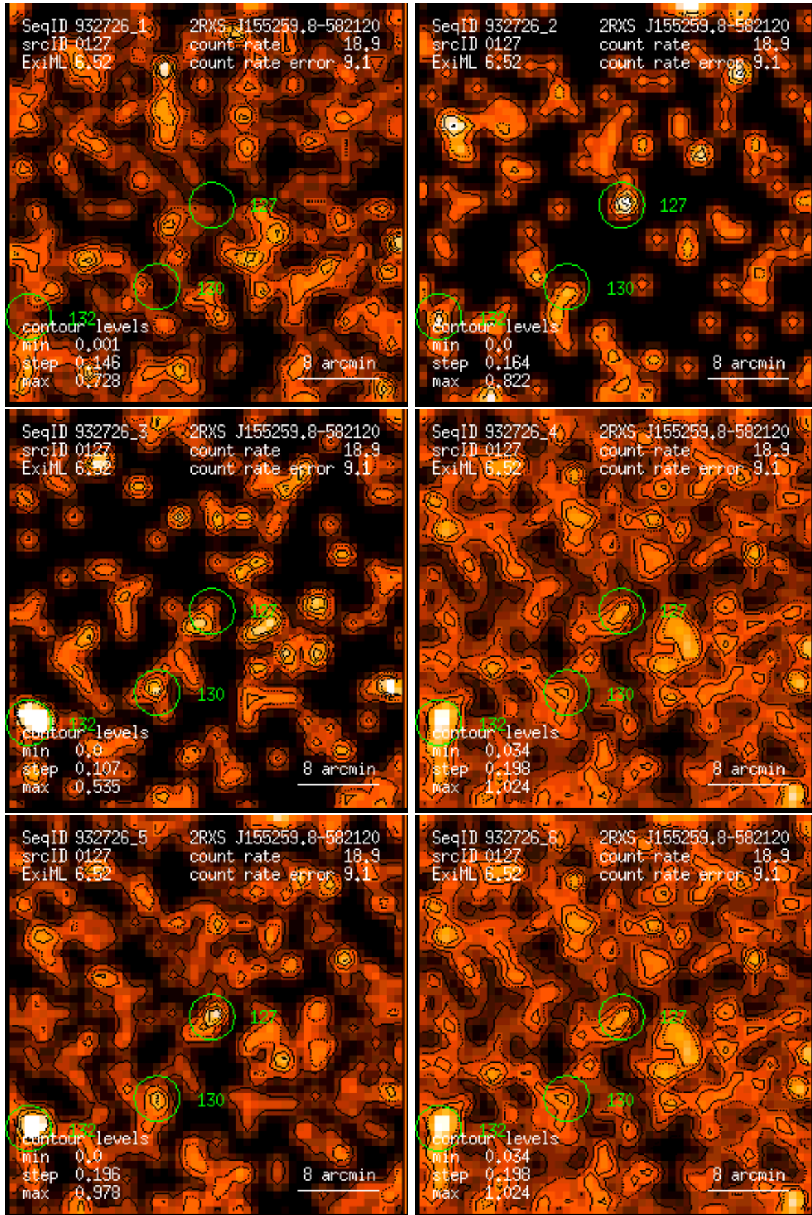
Figure 127: RASS 932726: detection 0127: band rate images, Gaussian filter: (1) PSPC channels 11 – 41, (2) 52 – 90, (3) 91 – 201, (4) 11 – 235, (5) 52 – 201, (6) 11 – 201. Broad band rates in counts/ks. Band rate contour levels in counts/ks/arcmin 2 .
