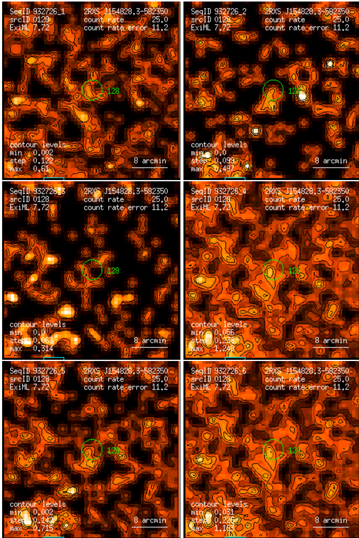
Figure 128: RASS 932726: detection 0128: band rate images, Gaussian filter: (1) PSPC channels 11 – 41, (2) 52 – 90, (3) 91 – 201, (4) 11 – 235, (5) 52 – 201, (6) 11 – 201. Broad band rates in counts/ks. Band rate contour levels in counts/ks/arcmin 2 .
