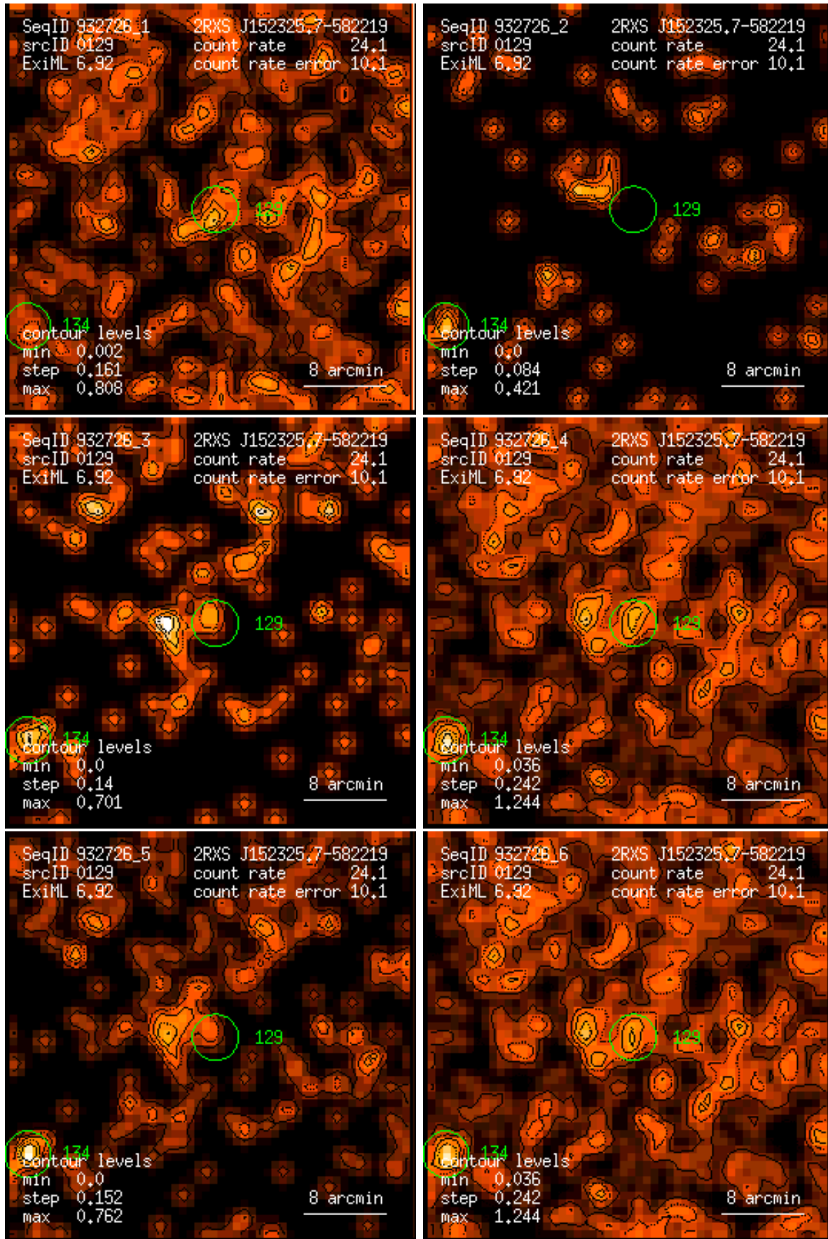
Figure 129: RASS 932726: detection 0129: band rate images, Gaussian filter: (1) PSPC channels 11 – 41, (2) 52 – 90, (3) 91 – 201, (4) 11 – 235, (5) 52 – 201, (6) 11 – 201. Broad band rates in counts/ks. Band rate contour levels in counts/ks/arcmin 2 .
