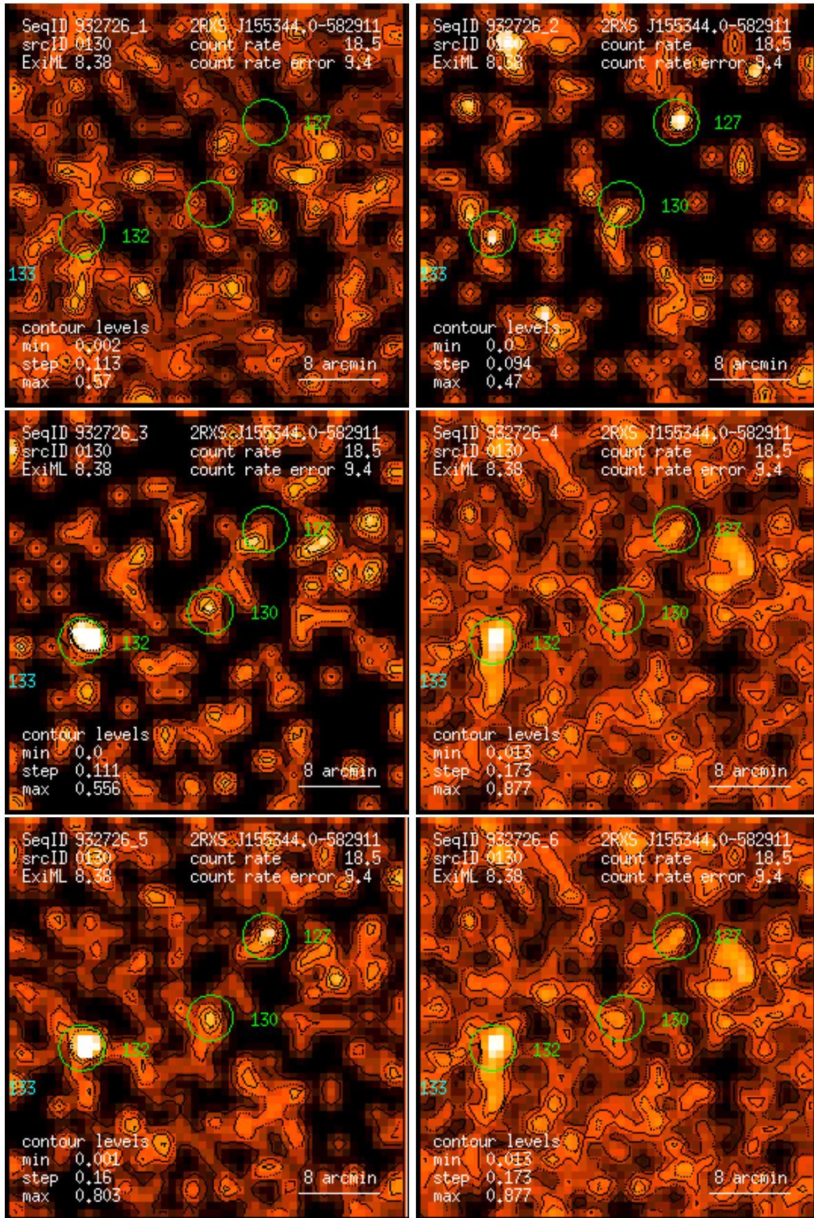
Figure 130: RASS 932726: detection 0130: band rate images, Gaussian filter: (1) PSPC channels 11 – 41, (2) 52 – 90, (3) 91 – 201, (4) 11 – 235, (5) 52 – 201, (6) 11 – 201. Broad band rates in counts/ks. Band rate contour levels in counts/ks/arcmin 2 .
