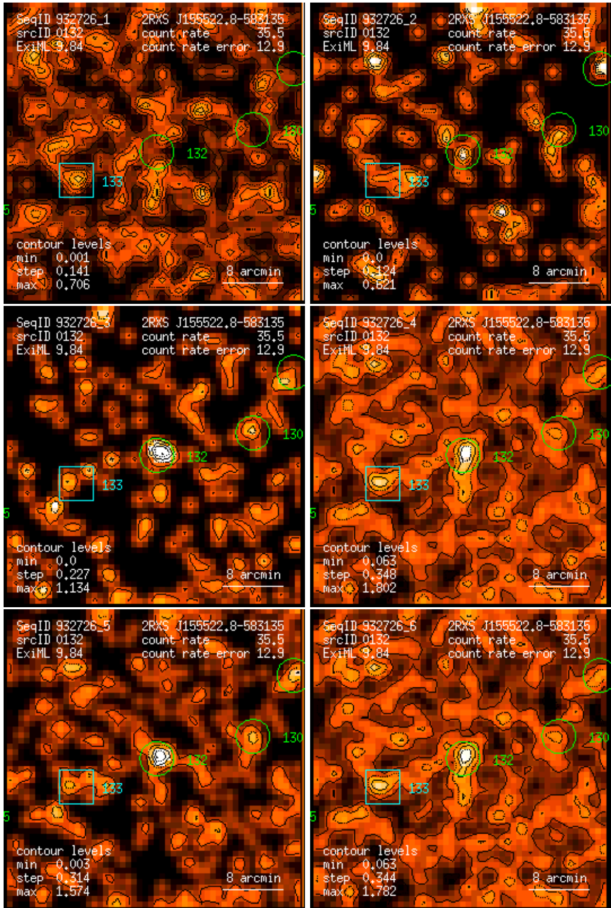
Figure 132: RASS 932726: detection 0132: band rate images, Gaussian filter: (1) PSPC channels 11 – 41, (2) 52 – 90, (3) 91 – 201, (4) 11 – 235, (5) 52 – 201, (6) 11 – 201. Broad band rates in counts/ks. Band rate contour levels in counts/ks/arcmin 2 .
