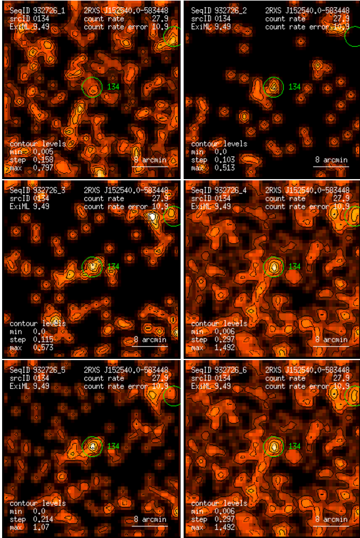
Figure 134: RASS 932726: detection 0134: band rate images, Gaussian filter: (1) PSPC channels 11 – 41, (2) 52 – 90, (3) 91 – 201, (4) 11 – 235, (5) 52 – 201, (6) 11 – 201. Broad band rates in counts/ks. Band rate contour levels in counts/ks/arcmin 2 .
