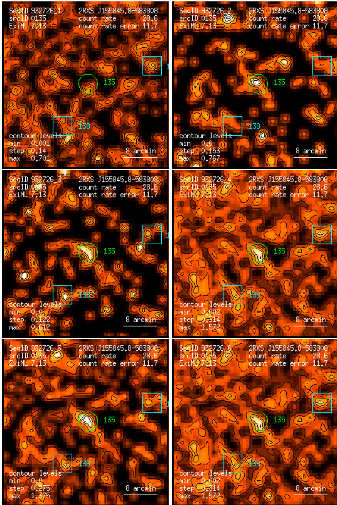
Figure 135: RASS 932726: detection 0135: band rate images, Gaussian filter: (1) PSPC channels 11 – 41, (2) 52 – 90, (3) 91 – 201, (4) 11 – 235, (5) 52 – 201, (6) 11 – 201. Broad band rates in counts/ks. Band rate contour levels in counts/ks/arcmin 2 .
