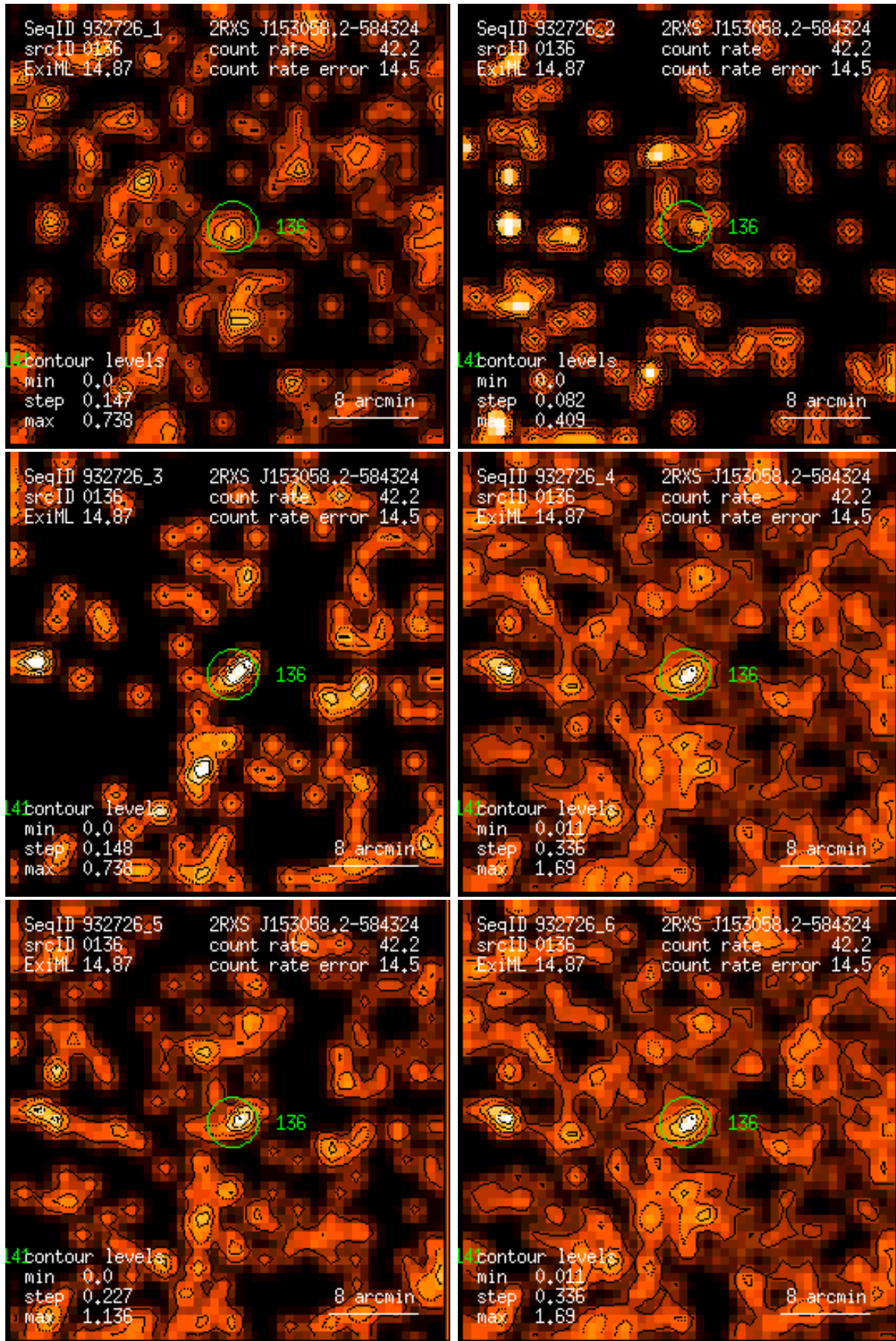
Figure 136: RASS 932726: detection 0136: band rate images, Gaussian filter: (1) PSPC channels 11 – 41, (2) 52 – 90, (3) 91 – 201, (4) 11 – 235, (5) 52 – 201, (6) 11 – 201. Broad band rates in counts/ks. Band rate contour levels in counts/ks/arcmin 2 .
