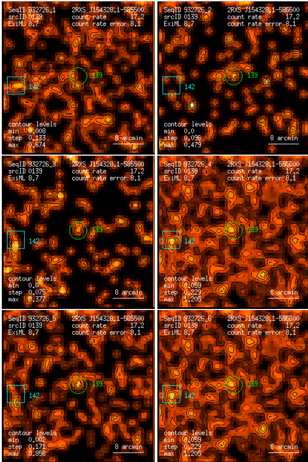
Figure 139: RASS 932726: detection 0139: band rate images, Gaussian filter: (1) PSPC channels 11 – 41, (2) 52 – 90, (3) 91 – 201, (4) 11 – 235, (5) 52 – 201, (6) 11 – 201. Broad band rates in counts/ks. Band rate contour levels in counts/ks/arcmin 2 .
