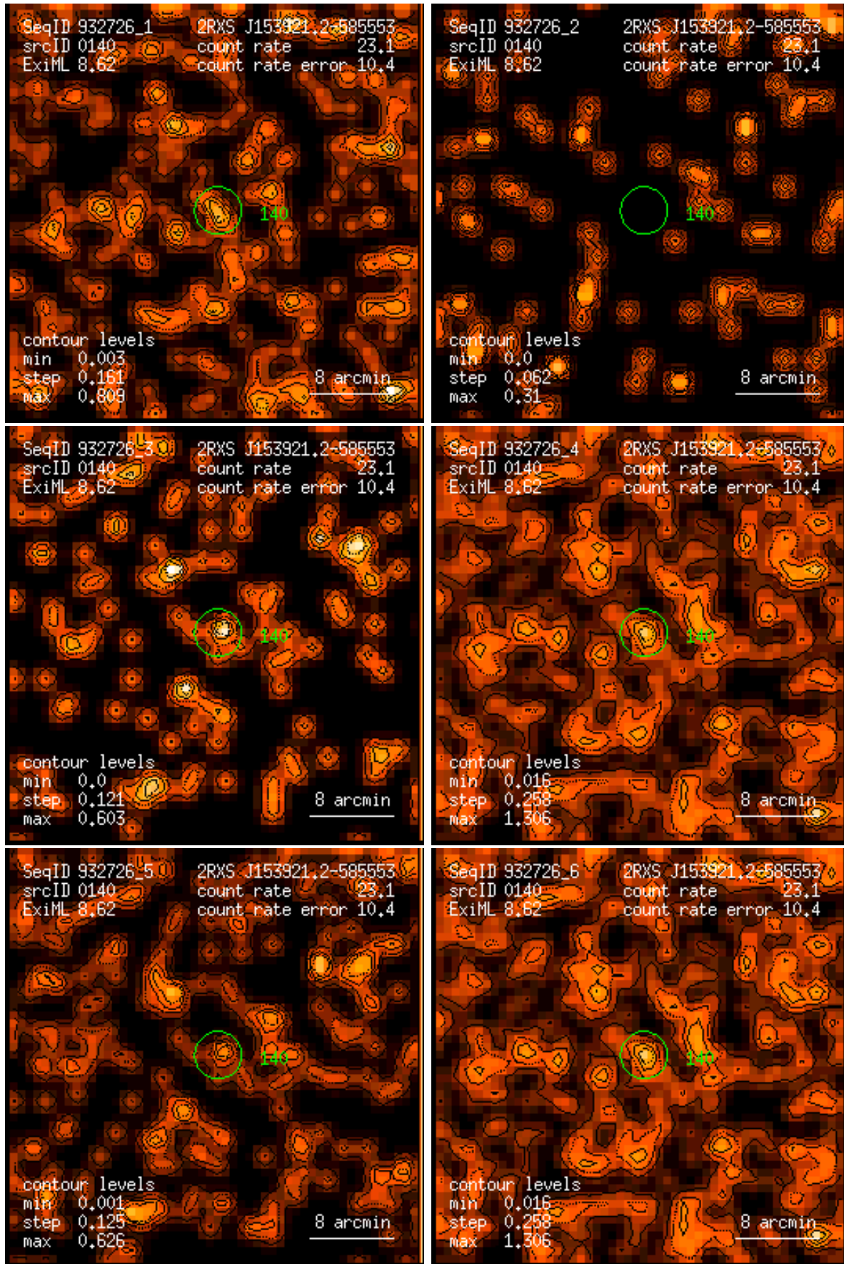
Figure 140: RASS 932726: detection 0140: band rate images, Gaussian filter: (1) PSPC channels 11 – 41, (2) 52 – 90, (3) 91 – 201, (4) 11 – 235, (5) 52 – 201, (6) 11 – 201. Broad band rates in counts/ks. Band rate contour levels in counts/ks/arcmin 2 .
