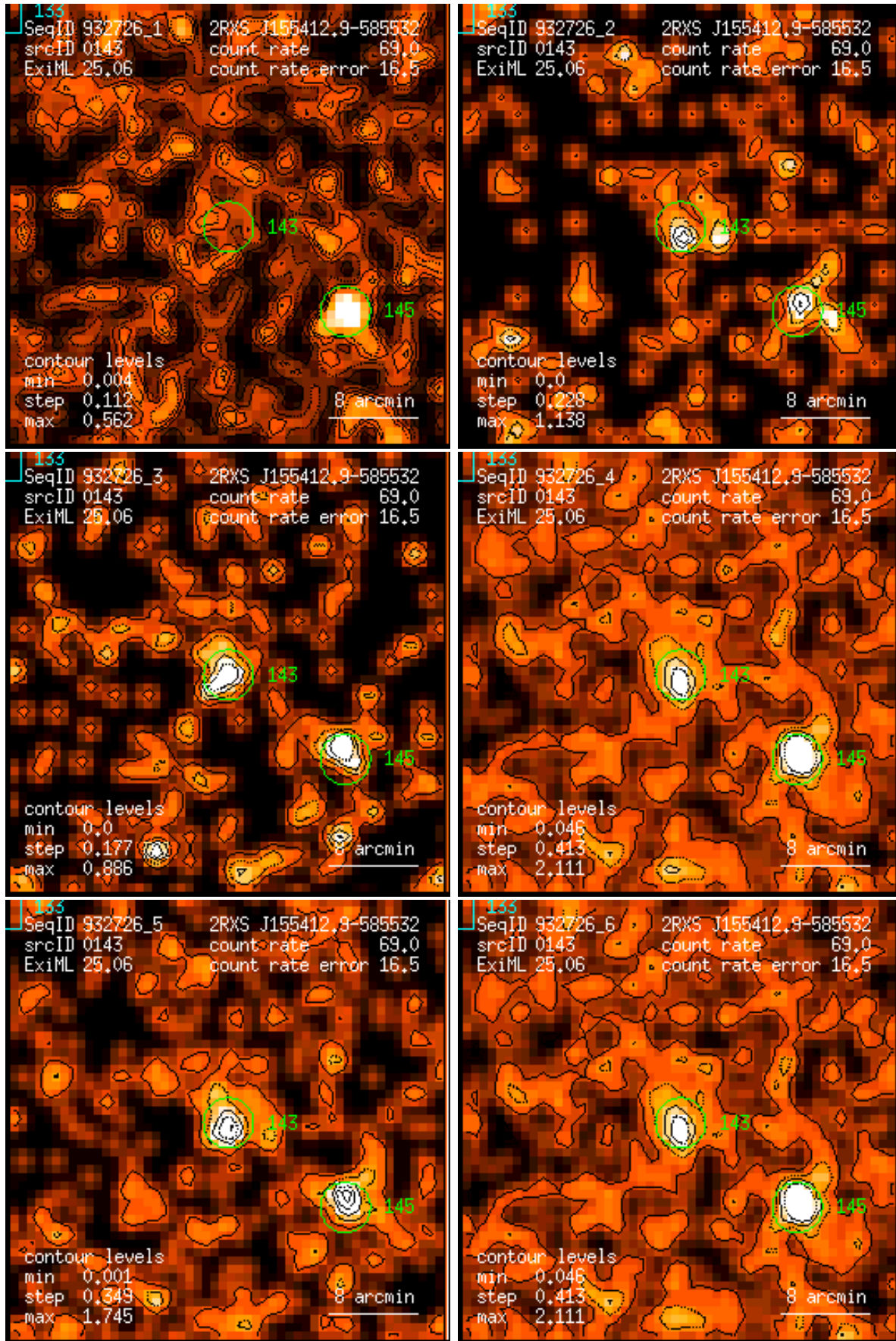
Figure 143: RASS 932726: detection 0143: band rate images, Gaussian filter: (1) PSPC channels 11 – 41, (2) 52 – 90, (3) 91 – 201, (4) 11 – 235, (5) 52 – 201, (6) 11 – 201. Broad band rates in counts/ks. Band rate contour levels in counts/ks/arcmin 2 .
