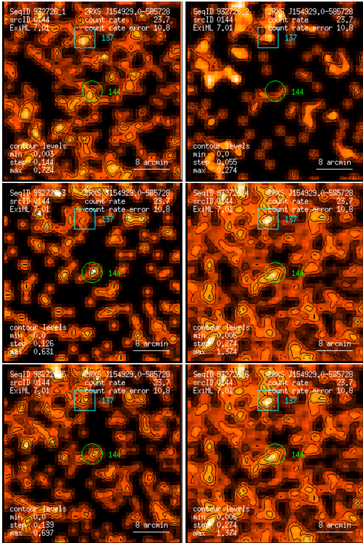
Figure 144: RASS 932726: detection 0144: band rate images, Gaussian filter: (1) PSPC channels 11 – 41, (2) 52 – 90, (3) 91 – 201, (4) 11 – 235, (5) 52 – 201, (6) 11 – 201. Broad band rates in counts/ks. Band rate contour levels in counts/ks/arcmin 2 .
