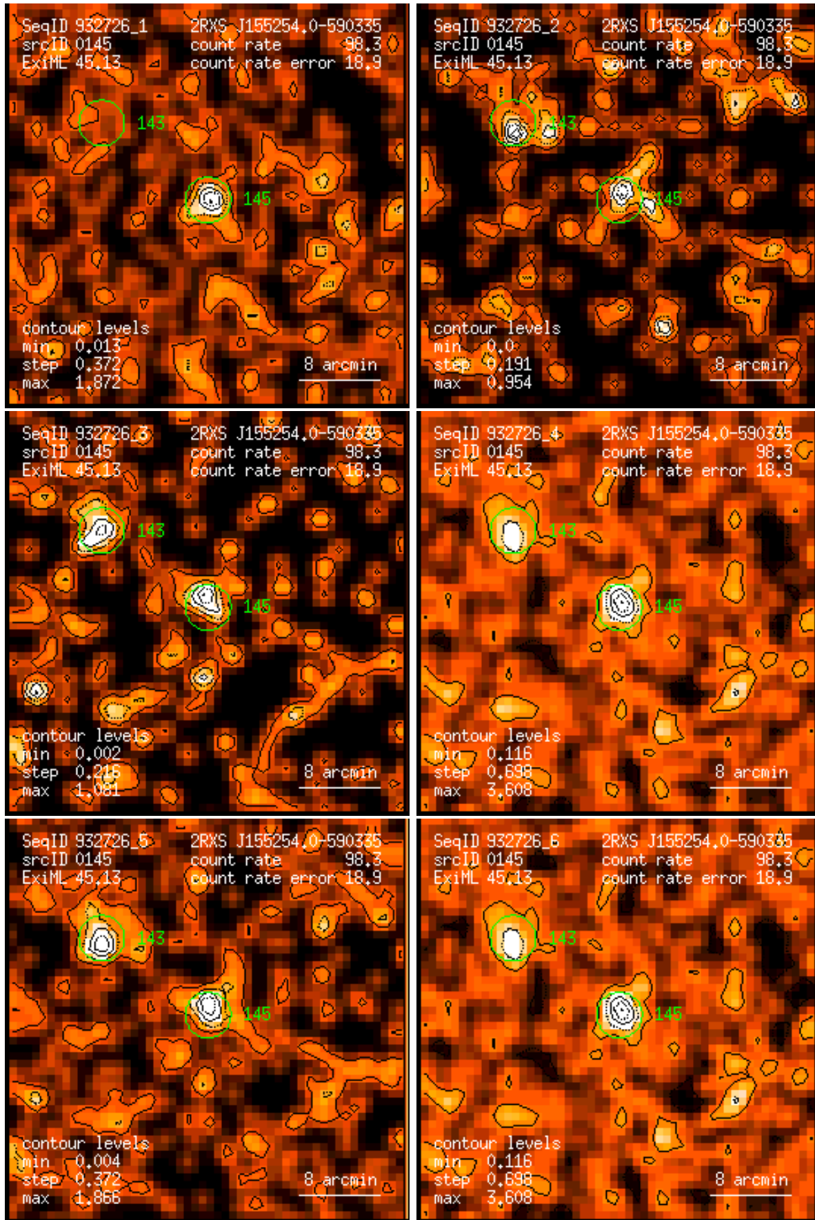
Figure 145: RASS 932726: detection 0145: band rate images, Gaussian filter: (1) PSPC channels 11 – 41, (2) 52 – 90, (3) 91 – 201, (4) 11 – 235, (5) 52 – 201, (6) 11 – 201. Broad band rates in counts/ks. Band rate contour levels in counts/ks/arcmin 2 .
