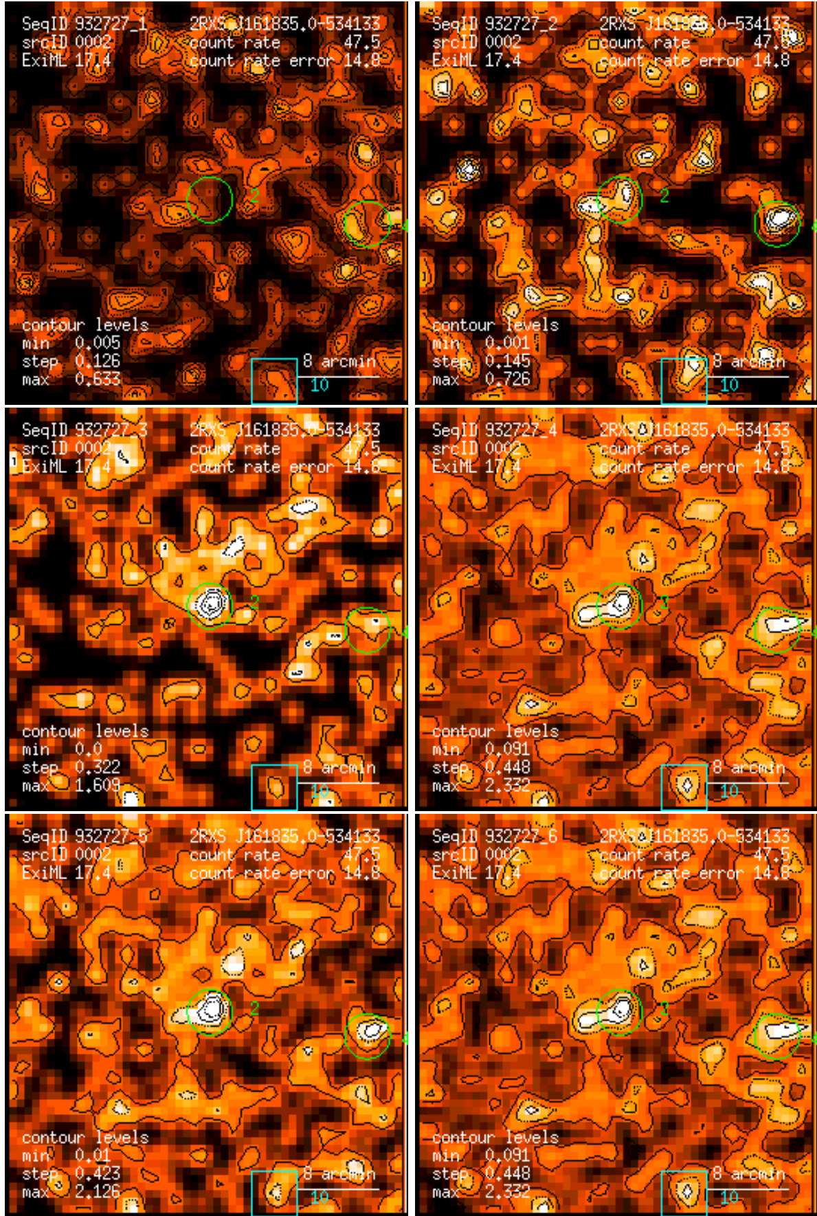
Figure 2: RASS 932727: detection 0002: band rate images, Gaussian filter: (1) PSPC channels 11 – 41, (2) 52 – 90, (3) 91 – 201, (4) 11 – 235, (5) 52 – 201, (6) 11 – 201. Broad band rates in counts/ks. Band rate contour levels in counts/ks/arcmin 2 .
