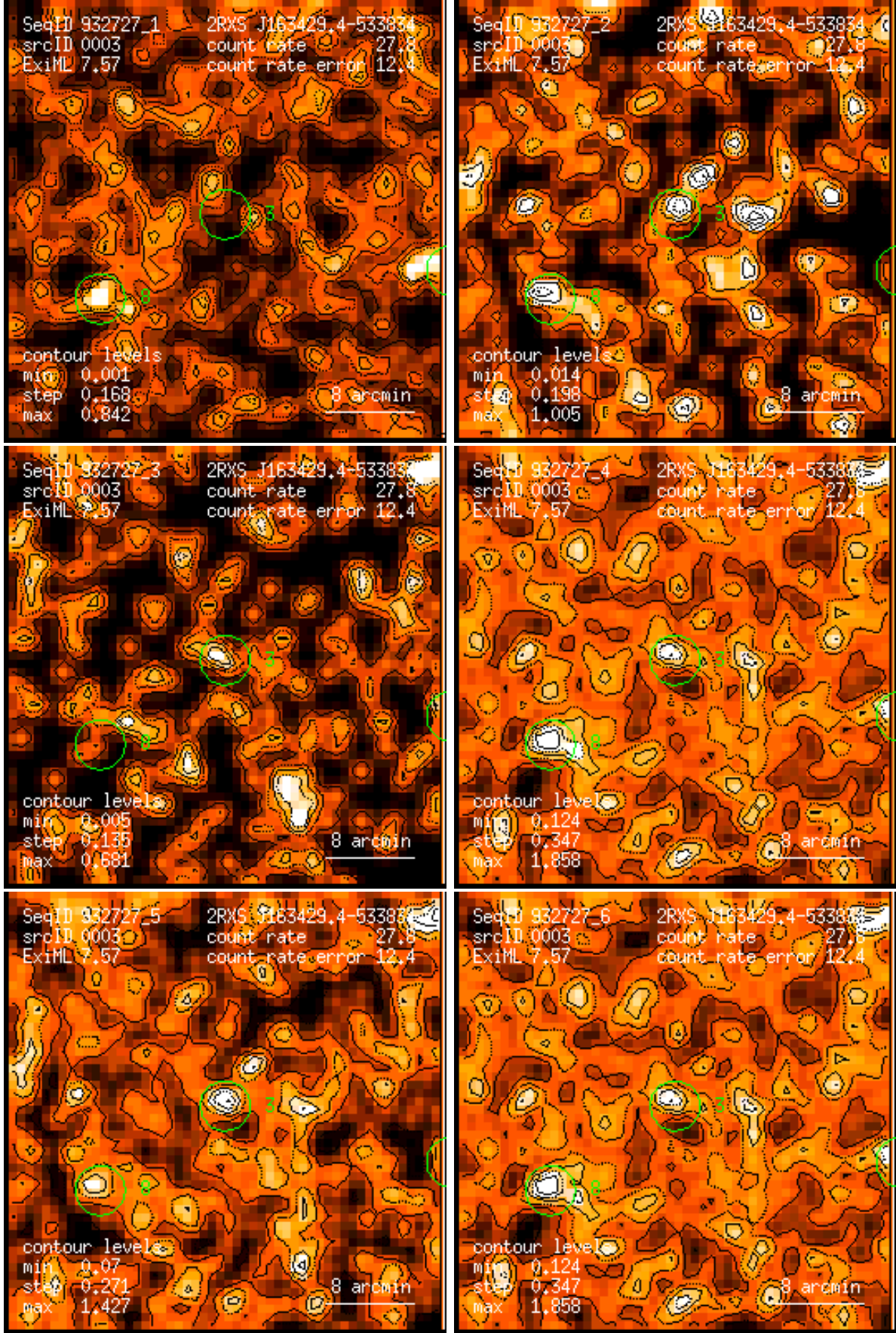
Figure 3: RASS 932727: detection 0003: band rate images, Gaussian filter: (1) PSPC channels 11 – 41, (2) 52 – 90, (3) 91 – 201, (4) 11 – 235, (5) 52 – 201, (6) 11 – 201. Broad band rates in counts/ks. Band rate contour levels in counts/ks/arcmin 2 .
