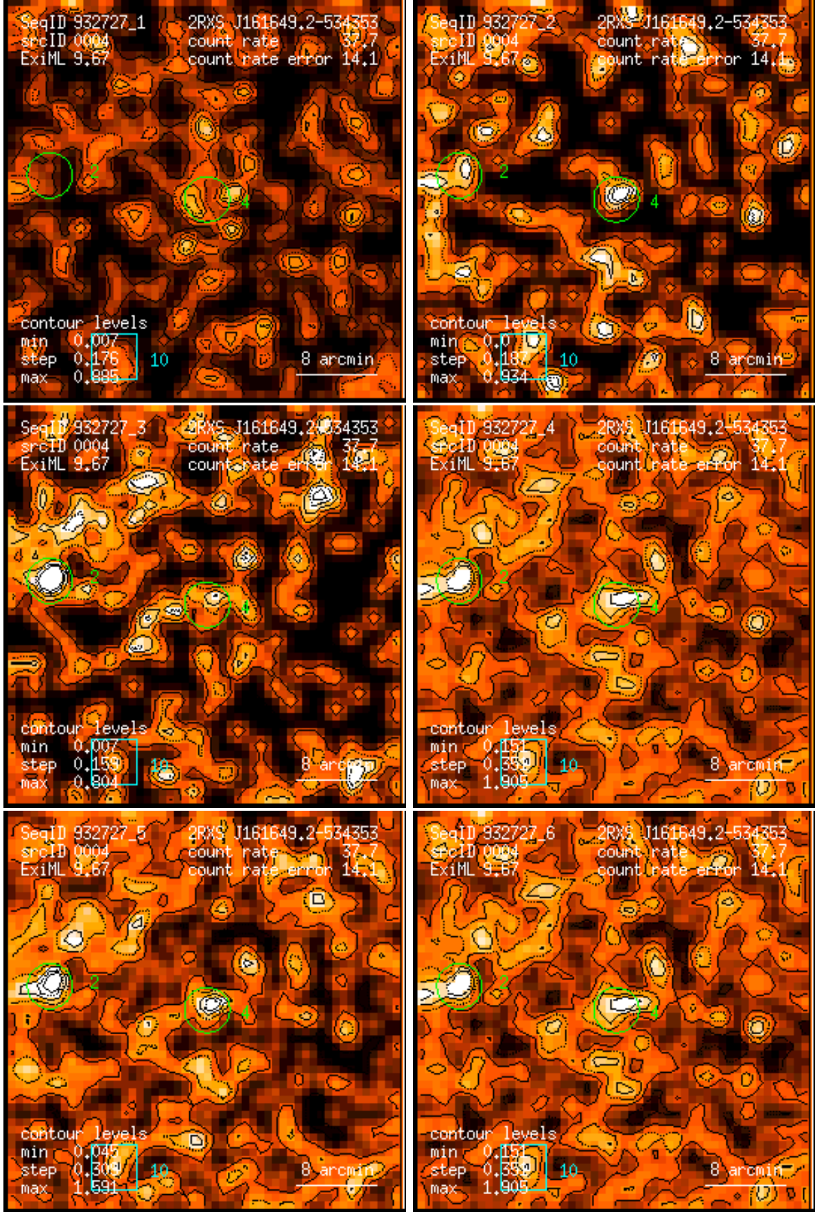
Figure 4: RASS 932727: detection 0004: band rate images, Gaussian filter: (1) PSPC channels 11 – 41, (2) 52 – 90, (3) 91 – 201, (4) 11 – 235, (5) 52 – 201, (6) 11 – 201. Broad band rates in counts/ks. Band rate contour levels in counts/ks/arcmin 2 .
