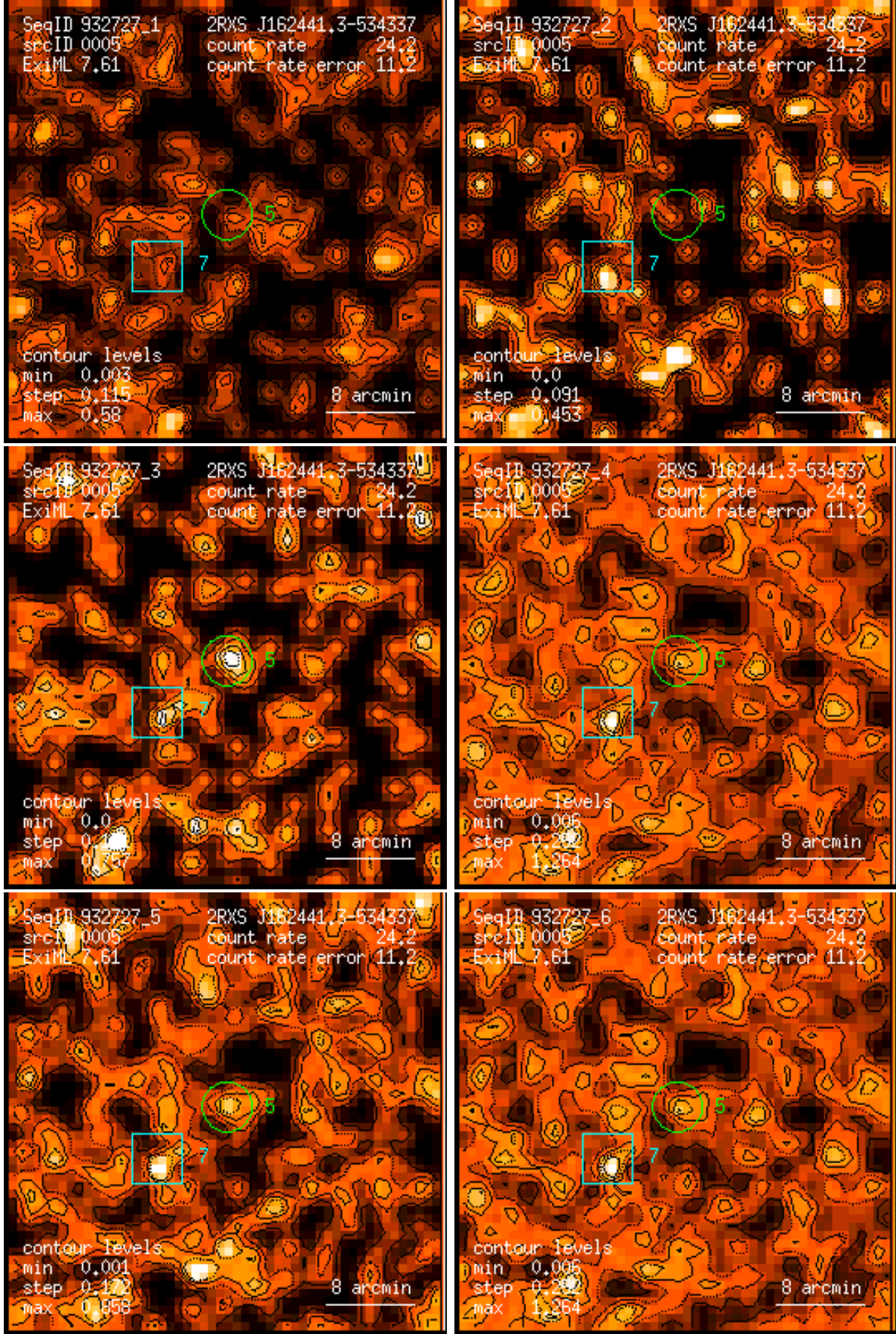
Figure 5: RASS 932727: detection 0005: band rate images, Gaussian filter: (1) PSPC channels 11 – 41, (2) 52 – 90, (3) 91 – 201, (4) 11 – 235, (5) 52 – 201, (6) 11 – 201. Broad band rates in counts/ks. Band rate contour levels in counts/ks/arcmin 2 .
