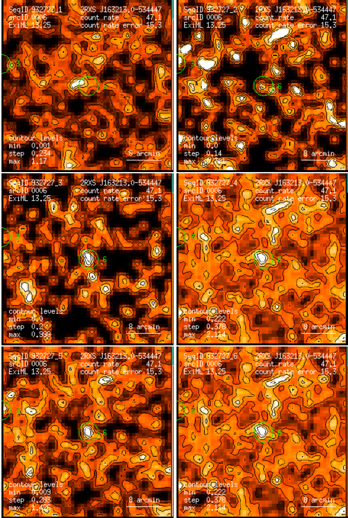
Figure 6: RASS 932727: detection 0006: band rate images, Gaussian filter: (1) PSPC channels 11 – 41, (2) 52 – 90, (3) 91 – 201, (4) 11 – 235, (5) 52 – 201, (6) 11 – 201. Broad band rates in counts/ks. Band rate contour levels in counts/ks/arcmin 2 .
