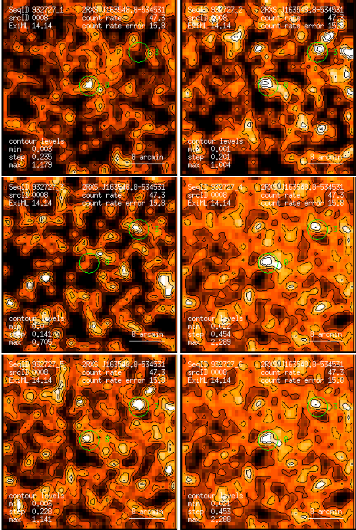
Figure 8: RASS 932727: detection 0008: band rate images, Gaussian filter: (1) PSPC channels 11 – 41, (2) 52 – 90, (3) 91 – 201, (4) 11 – 235, (5) 52 – 201, (6) 11 – 201. Broad band rates in counts/ks. Band rate contour levels in counts/ks/arcmin 2 .
