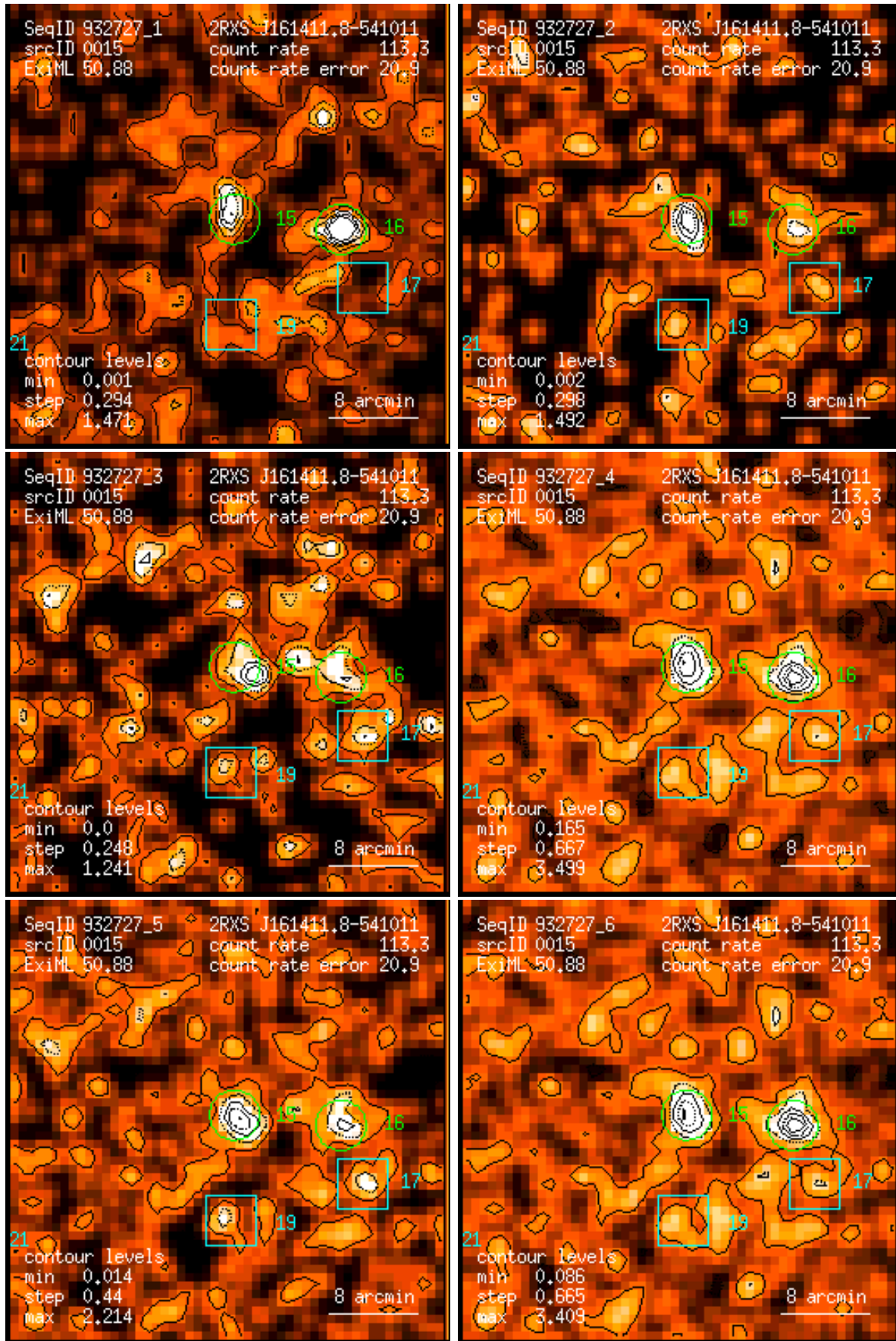
Figure 15: RASS 932727: detection 0015: band rate images, Gaussian filter: (1) PSPC channels 11 – 41, (2) 52 – 90, (3) 91 – 201, (4) 11 – 235, (5) 52 – 201, (6) 11 – 201. Broad band rates in counts/ks. Band rate contour levels in counts/ks/arcmin 2 .
