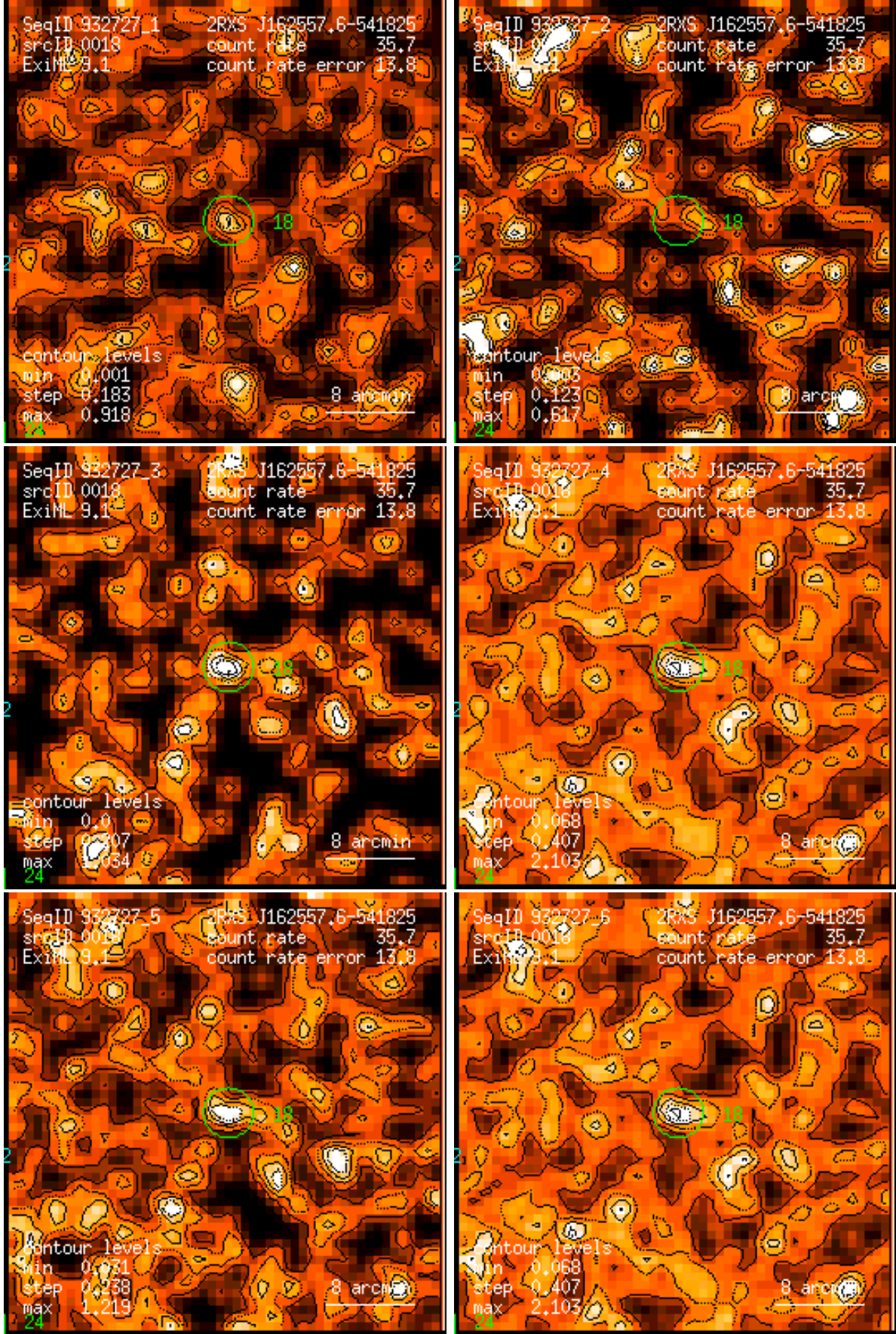
Figure 18: RASS 932727: detection 0018: band rate images, Gaussian filter: (1) PSPC channels 11 – 41, (2) 52 – 90, (3) 91 – 201, (4) 11 – 235, (5) 52 – 201, (6) 11 – 201. Broad band rates in counts/ks. Band rate contour levels in counts/ks/arcmin 2 .
