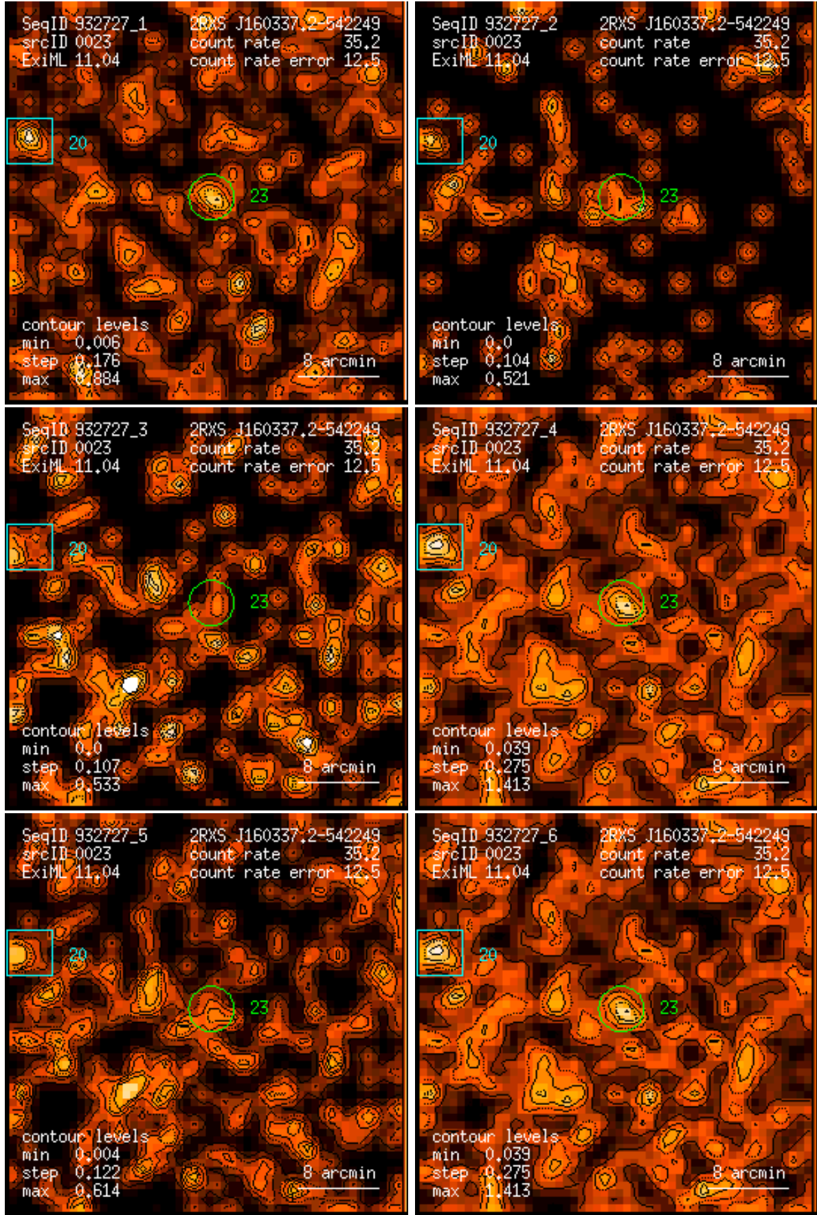
Figure 23: RASS 932727: detection 0023: band rate images, Gaussian filter: (1) PSPC channels 11 – 41, (2) 52 – 90, (3) 91 – 201, (4) 11 – 235, (5) 52 – 201, (6) 11 – 201. Broad band rates in counts/ks. Band rate contour levels in counts/ks/arcmin 2 .
