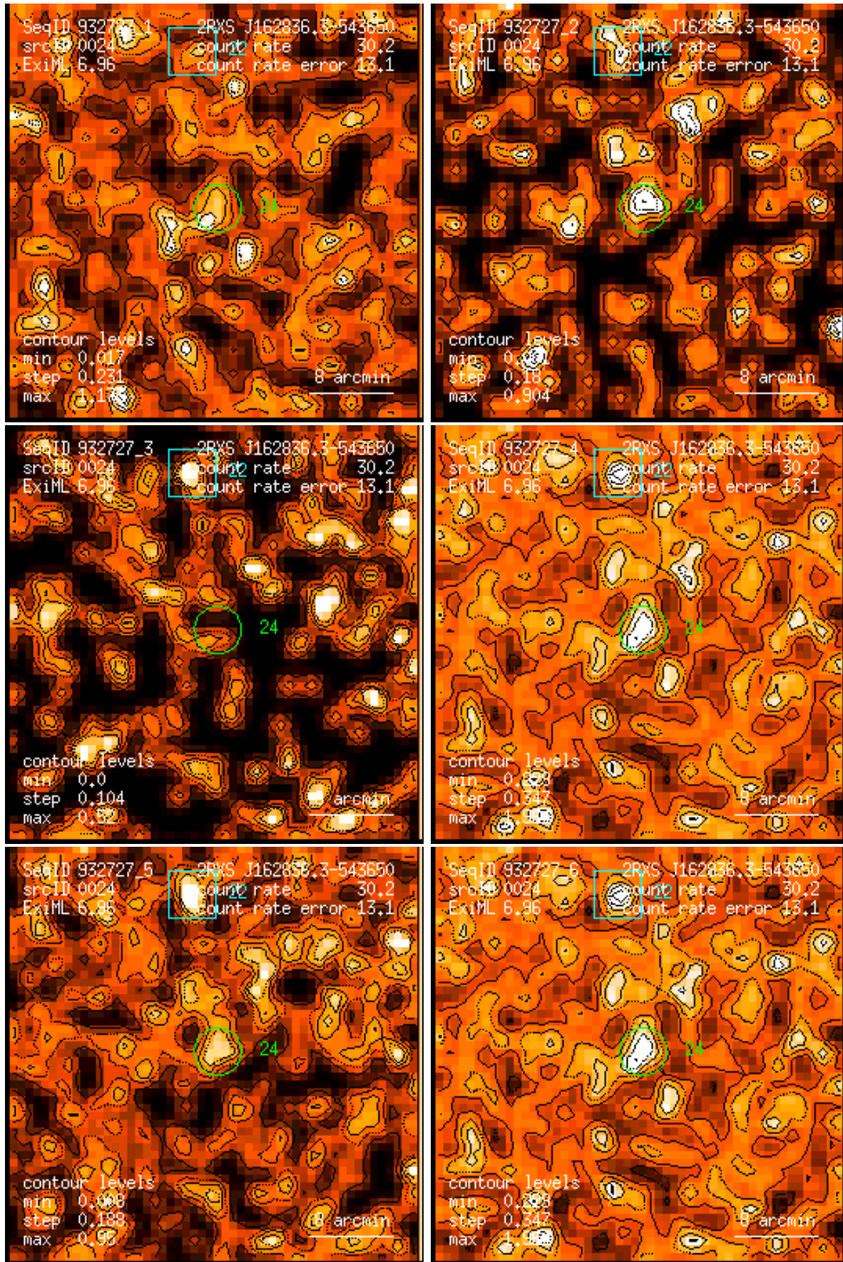
Figure 24: RASS 932727: detection 0024: band rate images, Gaussian filter: (1) PSPC channels 11 – 41, (2) 52 – 90, (3) 91 – 201, (4) 11 – 235, (5) 52 – 201, (6) 11 – 201. Broad band rates in counts/ks. Band rate contour levels in counts/ks/arcmin 2 .
