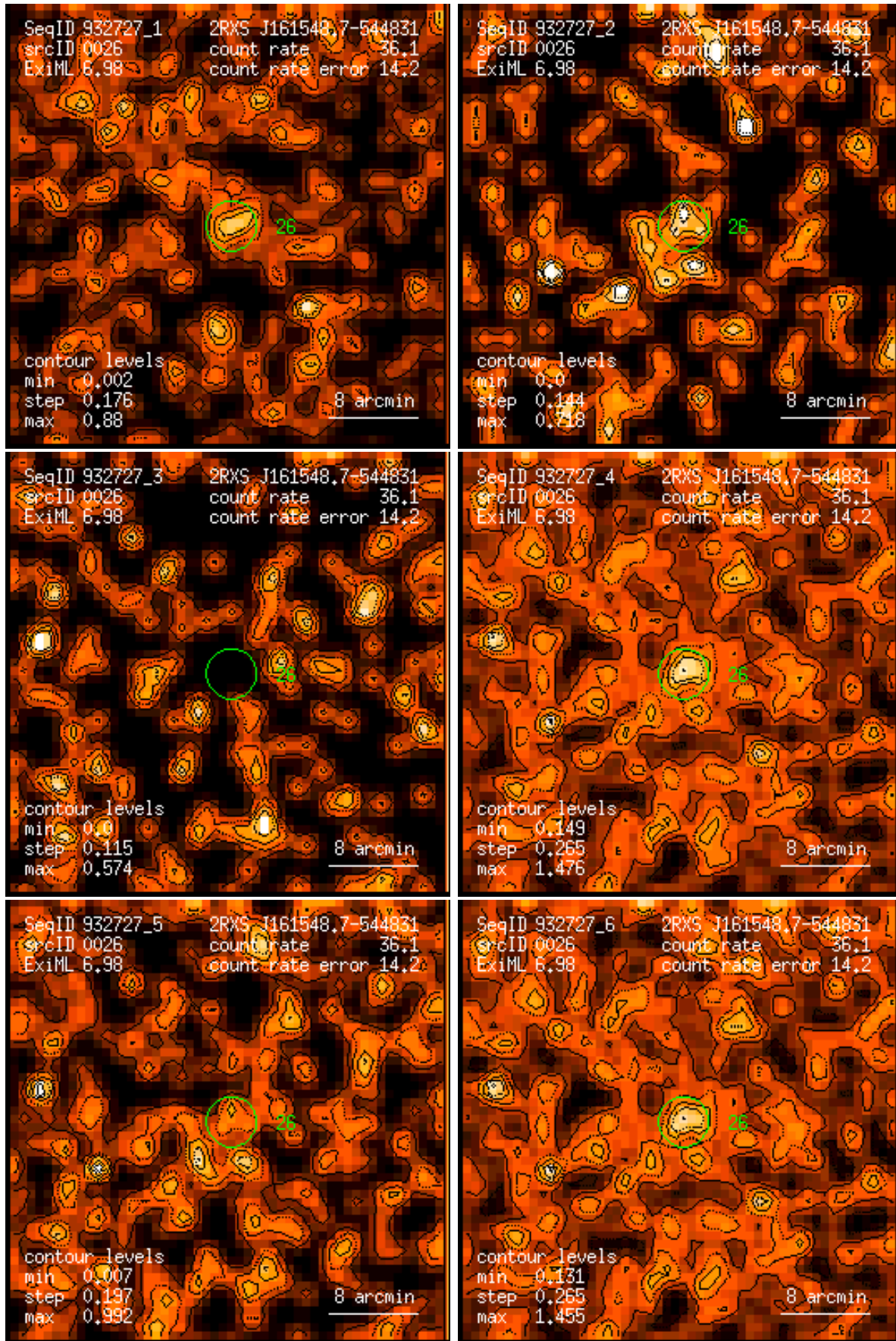
Figure 26: RASS 932727: detection 0026: band rate images, Gaussian filter: (1) PSPC channels 11 – 41, (2) 52 – 90, (3) 91 – 201, (4) 11 – 235, (5) 52 – 201, (6) 11 – 201. Broad band rates in counts/ks. Band rate contour levels in counts/ks/arcmin 2 .
