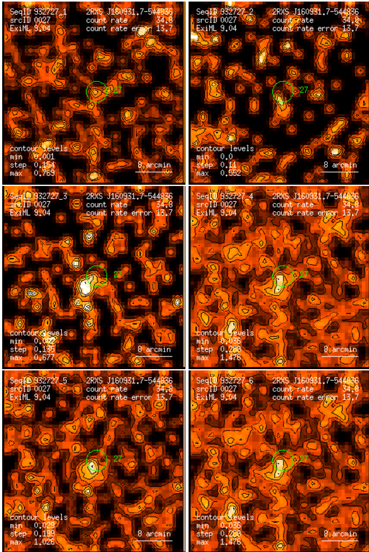
Figure 27: RASS 932727: detection 0027: band rate images, Gaussian filter: (1) PSPC channels 11 – 41, (2) 52 – 90, (3) 91 – 201, (4) 11 – 235, (5) 52 – 201, (6) 11 – 201. Broad band rates in counts/ks. Band rate contour levels in counts/ks/arcmin 2 .
