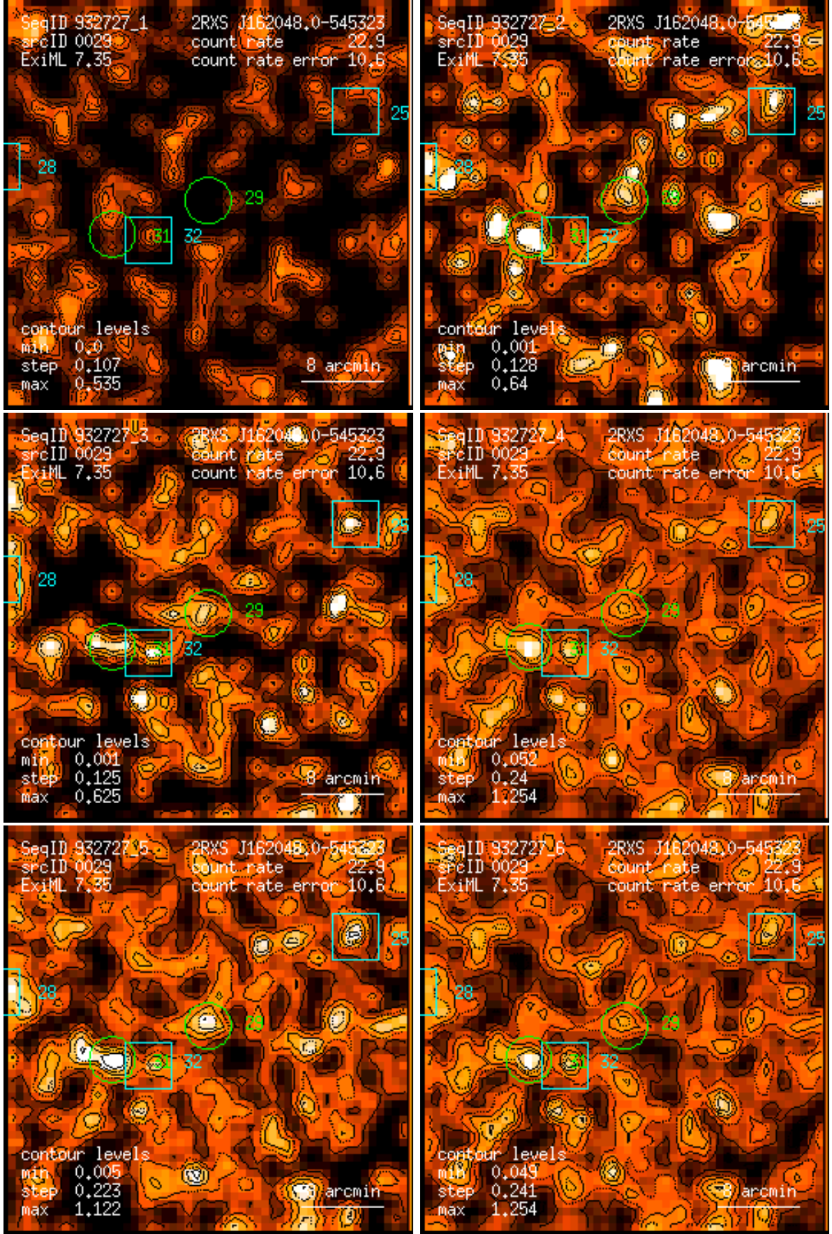
Figure 29: RASS 932727: detection 0029: band rate images, Gaussian filter: (1) PSPC channels 11 – 41, (2) 52 – 90, (3) 91 – 201, (4) 11 – 235, (5) 52 – 201, (6) 11 – 201. Broad band rates in counts/ks. Band rate contour levels in counts/ks/arcmin 2 .
