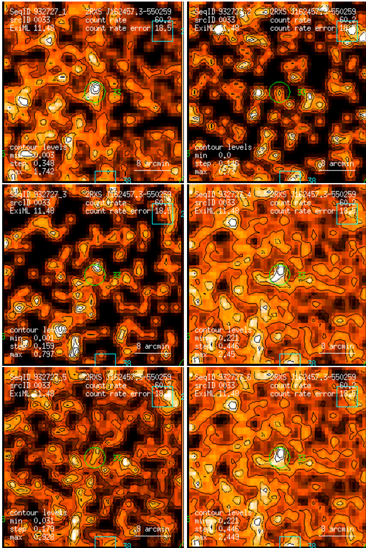
Figure 33: RASS 932727: detection 0033: band rate images, Gaussian filter: (1) PSPC channels 11 – 41, (2) 52 – 90, (3) 91 – 201, (4) 11 – 235, (5) 52 – 201, (6) 11 – 201. Broad band rates in counts/ks. Band rate contour levels in counts/ks/arcmin 2 .
