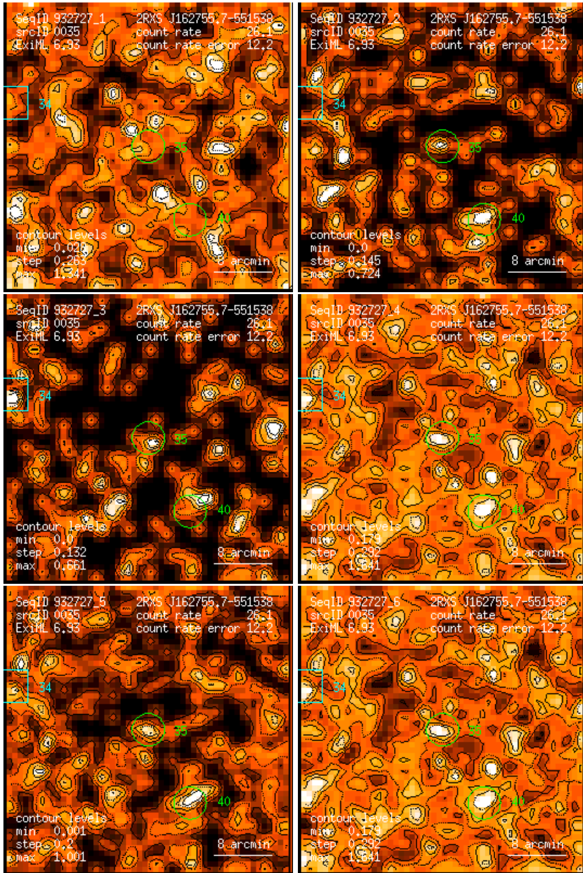
Figure 35: RASS 932727: detection 0035: band rate images, Gaussian filter: (1) PSPC channels 11 – 41, (2) 52 – 90, (3) 91 – 201, (4) 11 – 235, (5) 52 – 201, (6) 11 – 201. Broad band rates in counts/ks. Band rate contour levels in counts/ks/arcmin 2 .
