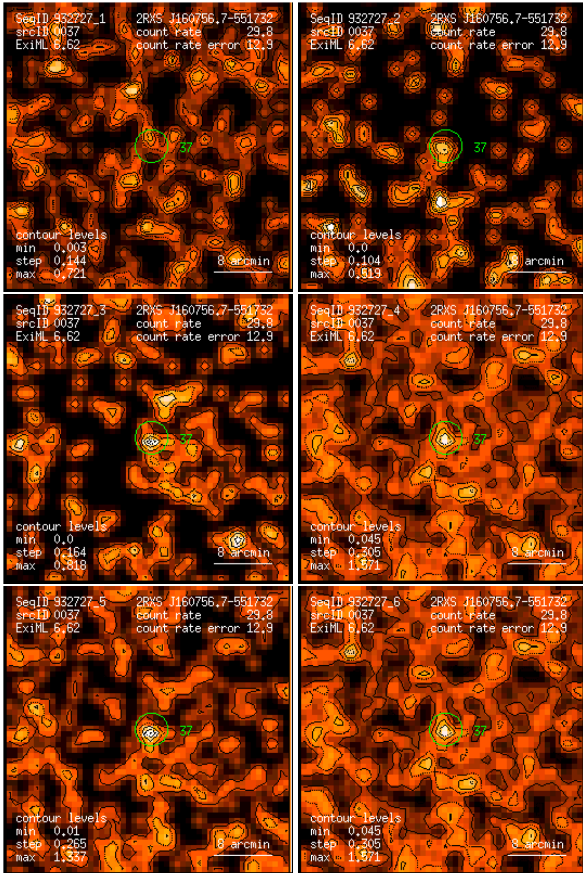
Figure 37: RASS 932727: detection 0037: band rate images, Gaussian filter: (1) PSPC channels 11 – 41, (2) 52 – 90, (3) 91 – 201, (4) 11 – 235, (5) 52 – 201, (6) 11 – 201. Broad band rates in counts/ks. Band rate contour levels in counts/ks/arcmin 2 .
