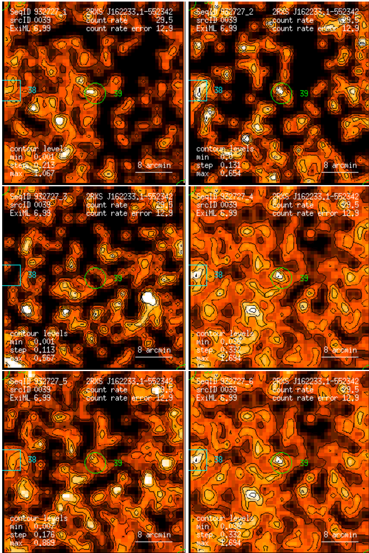
Figure 39: RASS 932727: detection 0039: band rate images, Gaussian filter: (1) PSPC channels 11 – 41, (2) 52 – 90, (3) 91 – 201, (4) 11 – 235, (5) 52 – 201, (6) 11 – 201. Broad band rates in counts/ks. Band rate contour levels in counts/ks/arcmin 2 .
