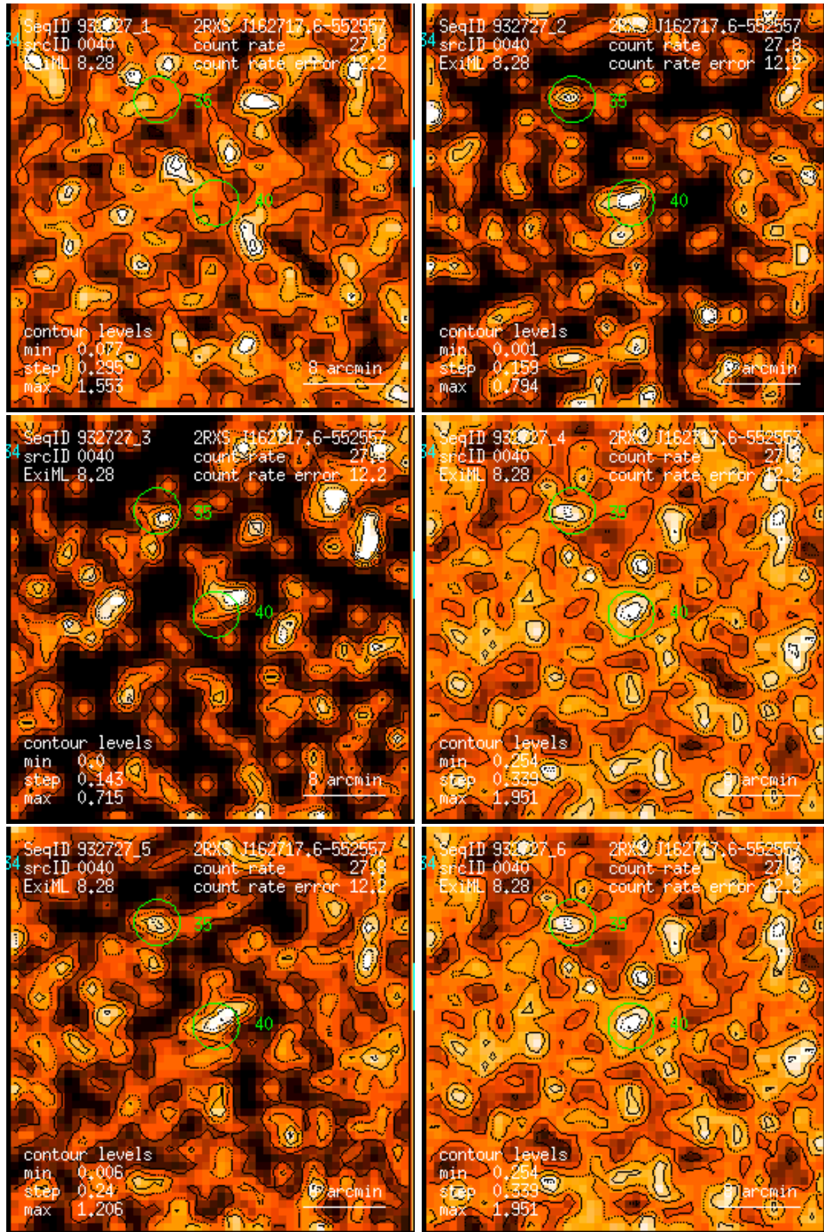
Figure 40: RASS 932727: detection 0040: band rate images, Gaussian filter: (1) PSPC channels 11 – 41, (2) 52 – 90, (3) 91 – 201, (4) 11 – 235, (5) 52 – 201, (6) 11 – 201. Broad band rates in counts/ks. Band rate contour levels in counts/ks/arcmin 2 .
