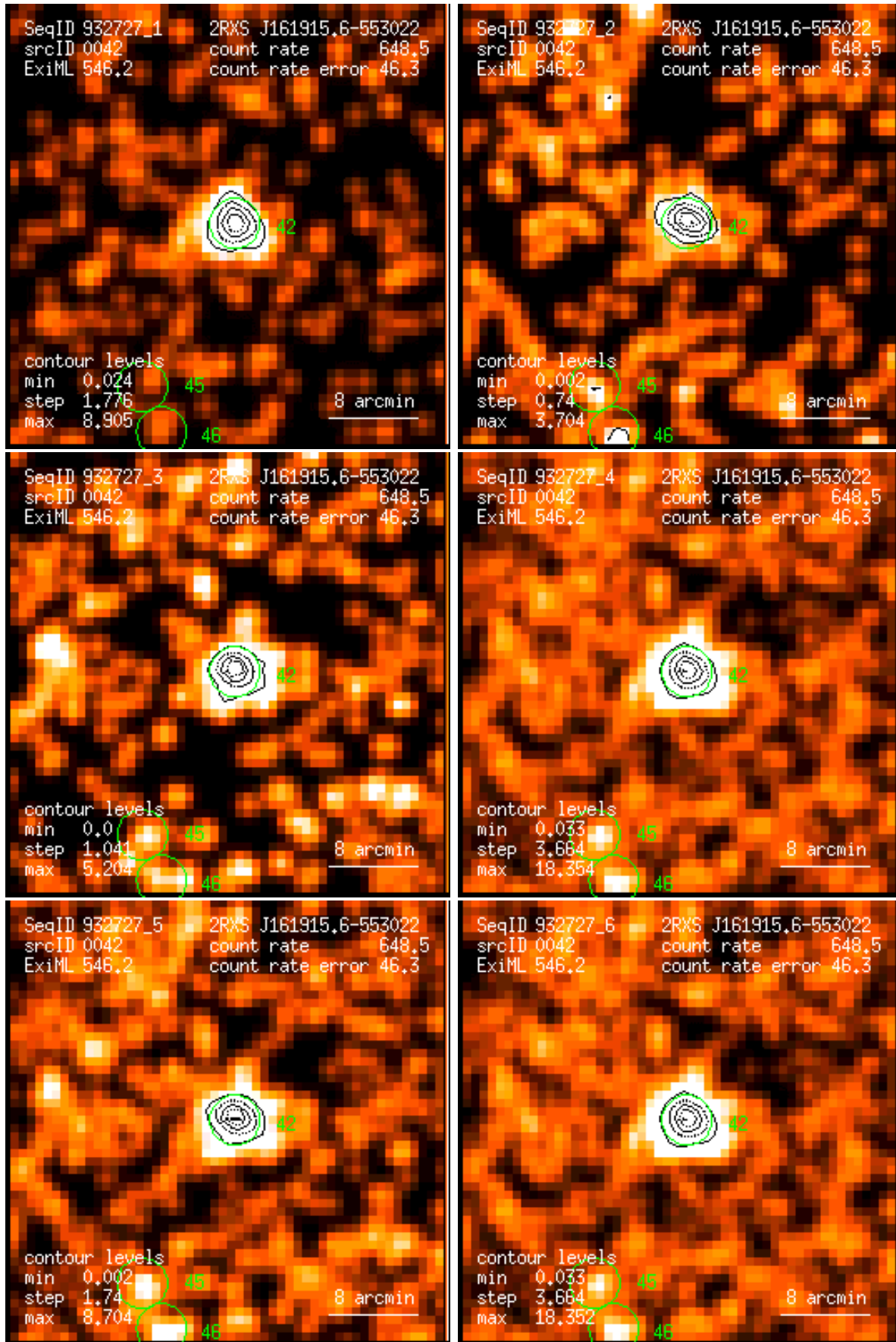
Figure 42: RASS 932727: detection 0042: band rate images, Gaussian filter: (1) PSPC channels 11 – 41, (2) 52 – 90, (3) 91 – 201, (4) 11 – 235, (5) 52 – 201, (6) 11 – 201. Broad band rates in counts/ks. Band rate contour levels in counts/ks/arcmin 2 .
