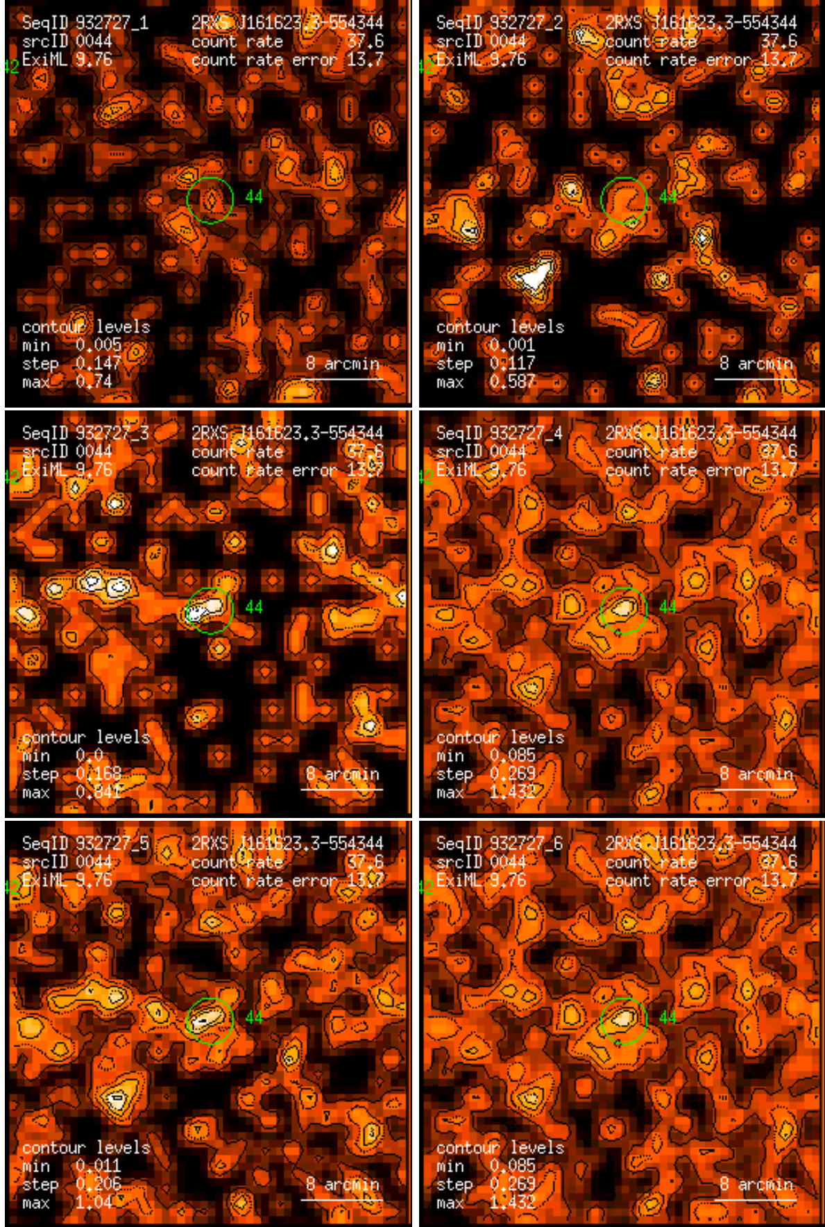
Figure 44: RASS 932727: detection 0044: band rate images, Gaussian filter: (1) PSPC channels 11 – 41, (2) 52 – 90, (3) 91 – 201, (4) 11 – 235, (5) 52 – 201, (6) 11 – 201. Broad band rates in counts/ks. Band rate contour levels in counts/ks/arcmin 2 .
