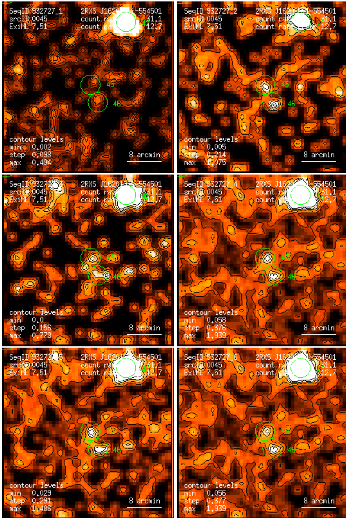
Figure 45: RASS 932727: detection 0045: band rate images, Gaussian filter: (1) PSPC channels 11 – 41, (2) 52 – 90, (3) 91 – 201, (4) 11 – 235, (5) 52 – 201, (6) 11 – 201. Broad band rates in counts/ks. Band rate contour levels in counts/ks/arcmin 2 .
