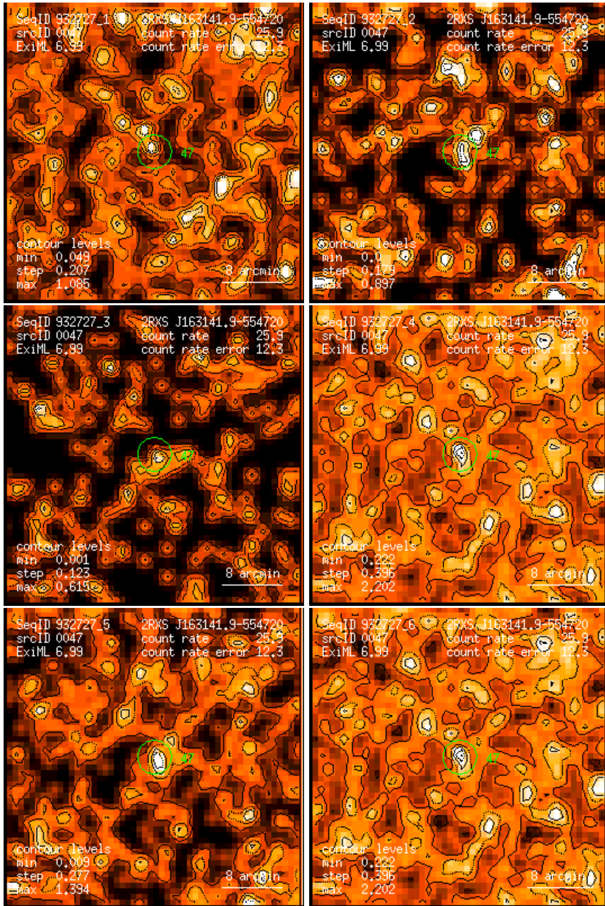
Figure 47: RASS 932727: detection 0047: band rate images, Gaussian filter: (1) PSPC channels 11 – 41, (2) 52 – 90, (3) 91 – 201, (4) 11 – 235, (5) 52 – 201, (6) 11 – 201. Broad band rates in counts/ks. Band rate contour levels in counts/ks/arcmin 2 .
