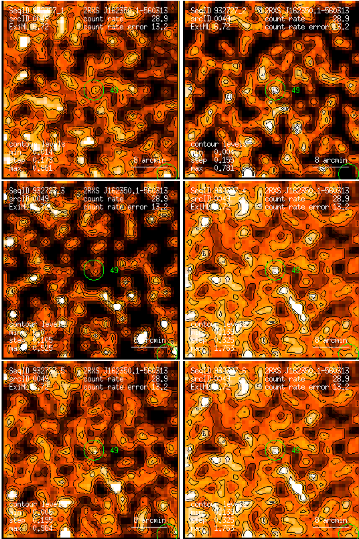
Figure 49: RASS 932727: detection 0049: band rate images, Gaussian filter: (1) PSPC channels 11 – 41, (2) 52 – 90, (3) 91 – 201, (4) 11 – 235, (5) 52 – 201, (6) 11 – 201. Broad band rates in counts/ks. Band rate contour levels in counts/ks/arcmin 2 .
