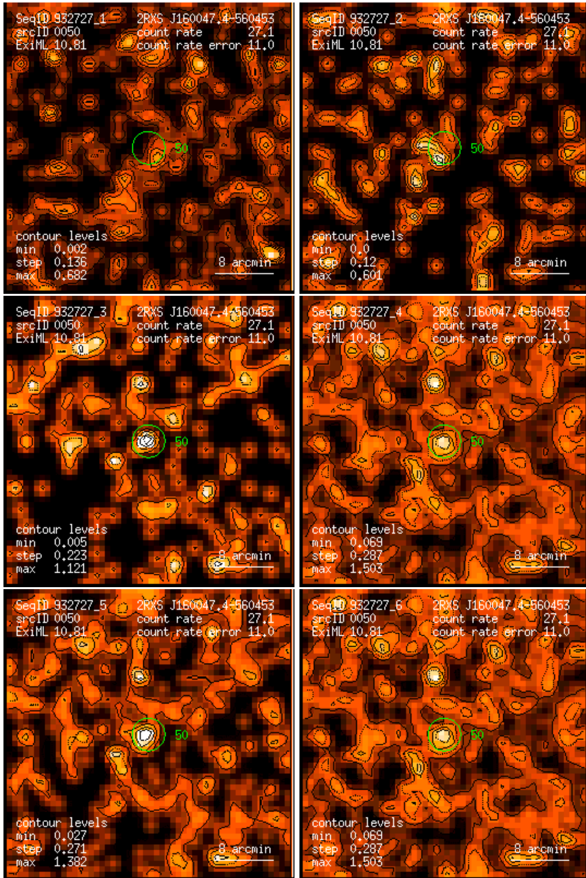
Figure 50: RASS 932727: detection 0050: band rate images, Gaussian filter: (1) PSPC channels 11 – 41, (2) 52 – 90, (3) 91 – 201, (4) 11 – 235, (5) 52 – 201, (6) 11 – 201. Broad band rates in counts/ks. Band rate contour levels in counts/ks/arcmin 2 .
