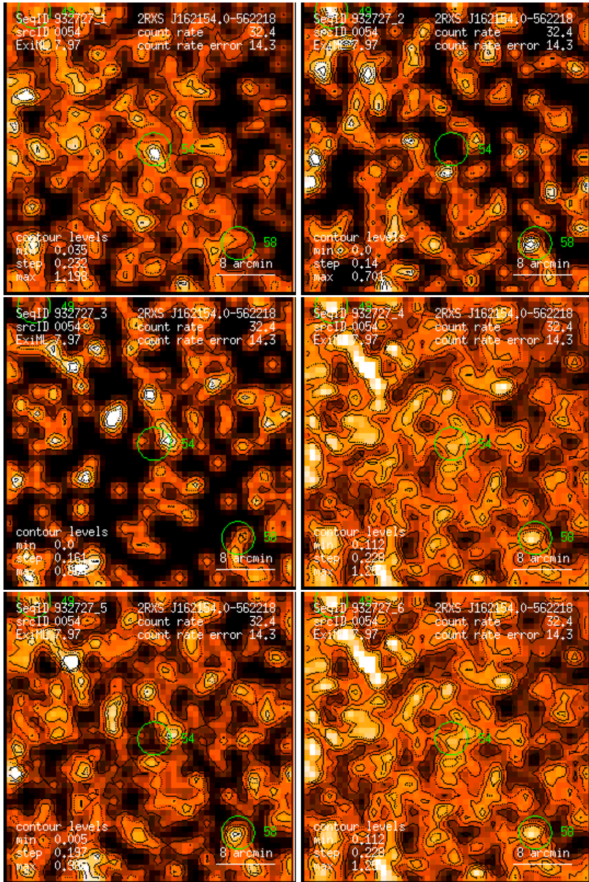
Figure 54: RASS 932727: detection 0054: band rate images, Gaussian filter: (1) PSPC channels 11 – 41, (2) 52 – 90, (3) 91 – 201, (4) 11 – 235, (5) 52 – 201, (6) 11 – 201. Broad band rates in counts/ks. Band rate contour levels in counts/ks/arcmin 2 .
